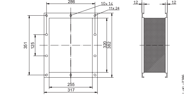
Flex. Druckstutzen / Flex. connector at outlet
