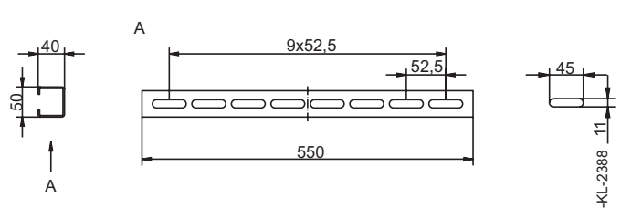
Profilschiene / Profile
