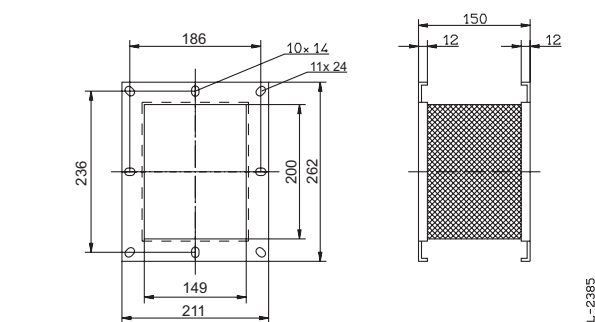
Flex. Druckstutzen / Flex. connector at outlet
