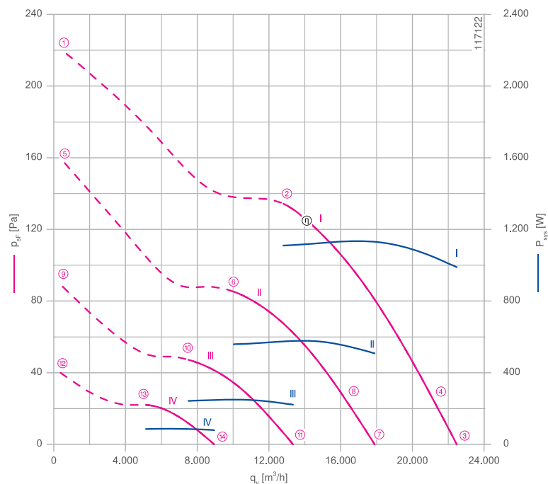
Characteristic curve
