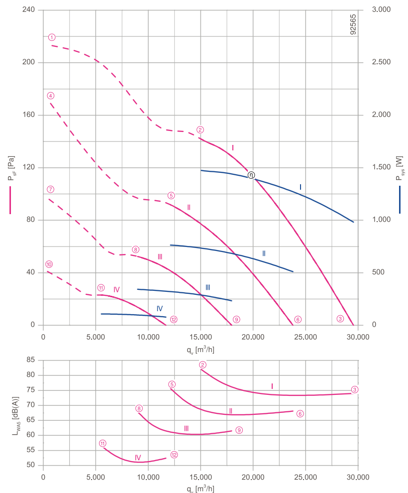
Characteristic curve
