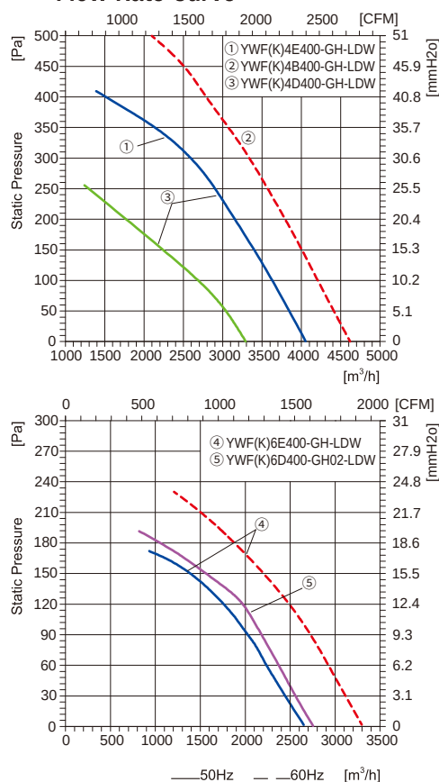
Flow Rate Curve
