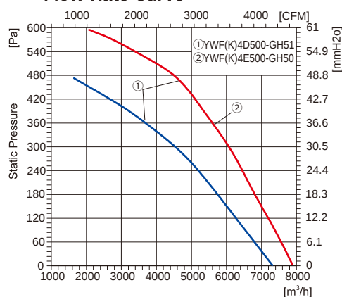
Flow Rate Curve
