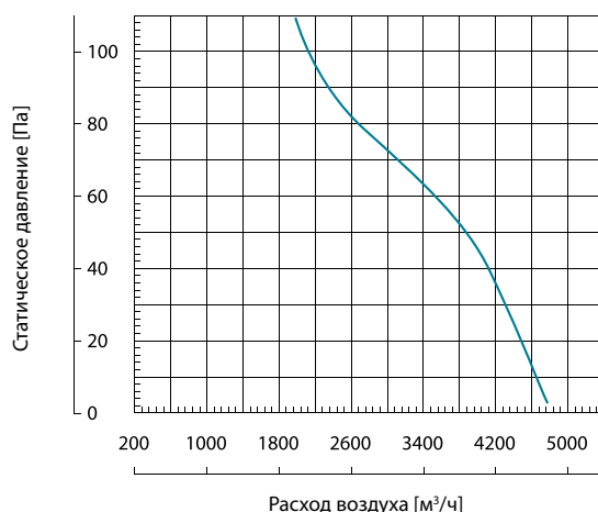
AX-W-450-4D, AX-D-450-4D
