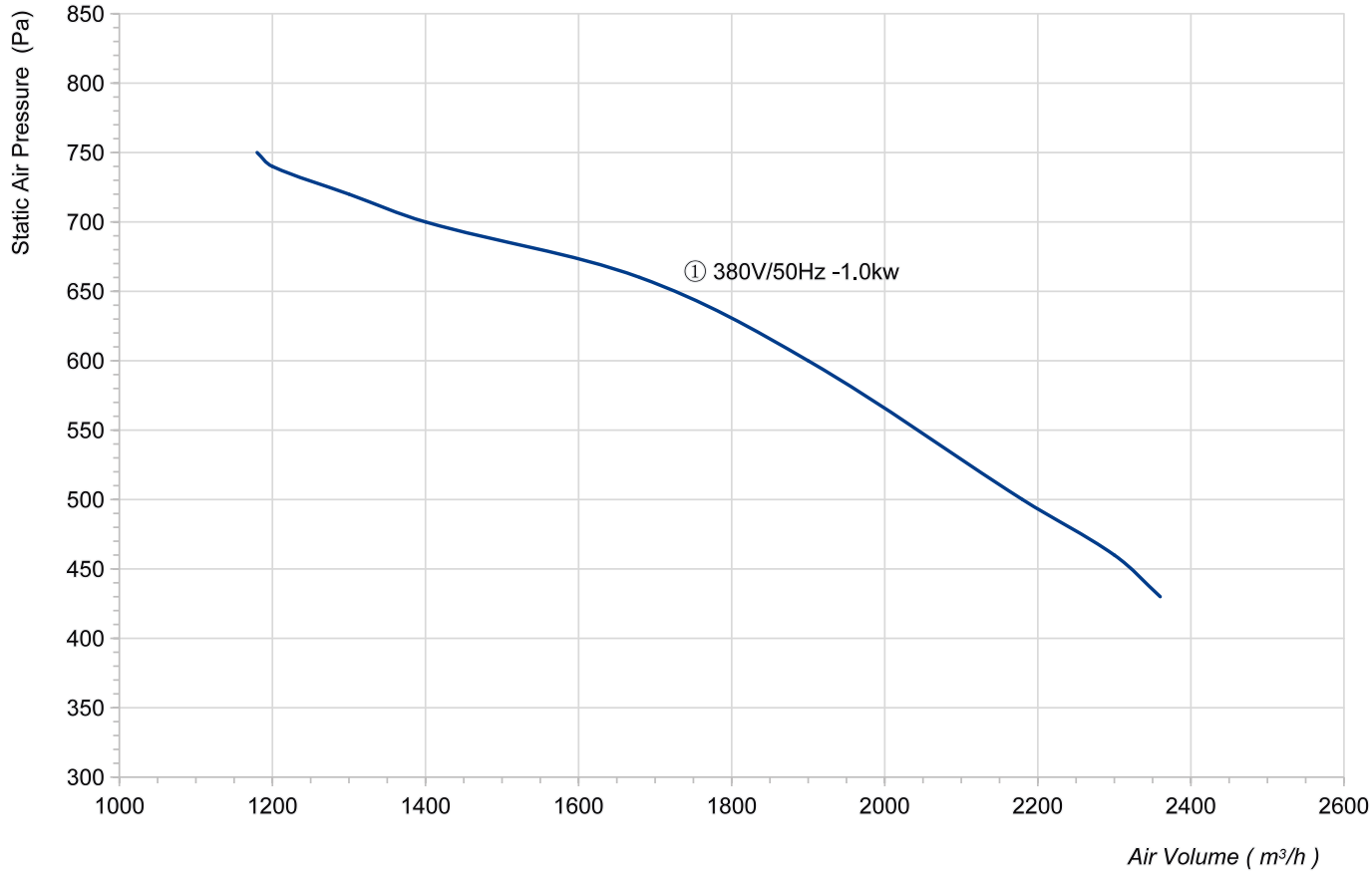
P-Q Curve
