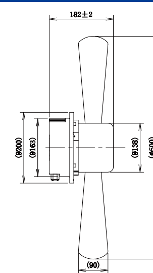
LWAE3G500TT-5MNW-02(Blowing)
