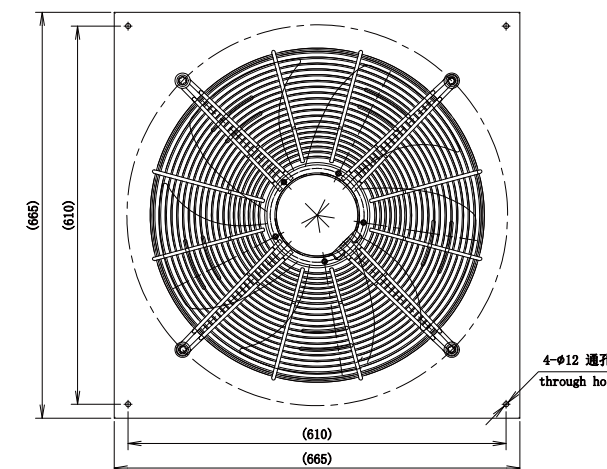
LWAE3G500TS-5MKW-05(Suction)
