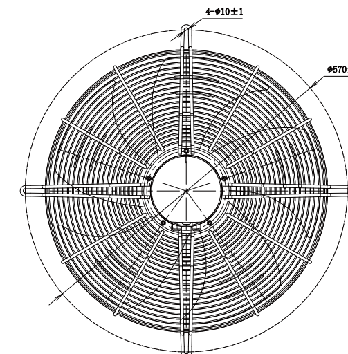
LWAE3G500TS-5MKW-05(Suction)
