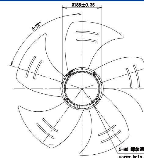
LWAE3G500TS-5MNW-01(Suction)
