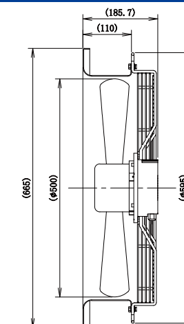
LWAE3G500TT-5MKW-06(Blowing)
