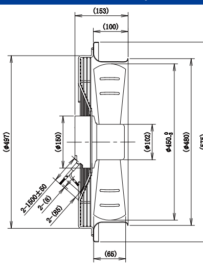
LWAE3G450ST-5MGW-06(Blowing)
