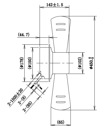
LWAE3G450ST-5MNW-02(Blowing)
