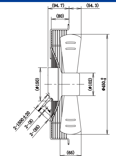
LWAE3G450ST-5MEW-04(Blowing)
