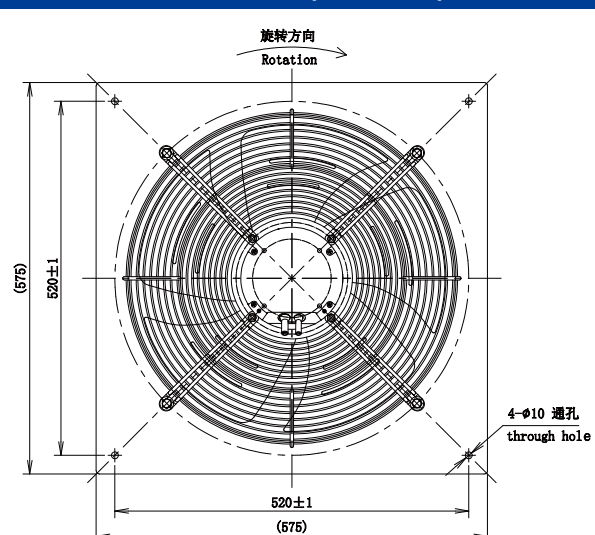
LWAE3G450SS-5MGW-05(Suction)
