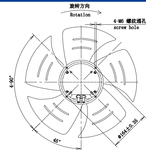
LWAE3G450SS-5MNW-01(Suction)
