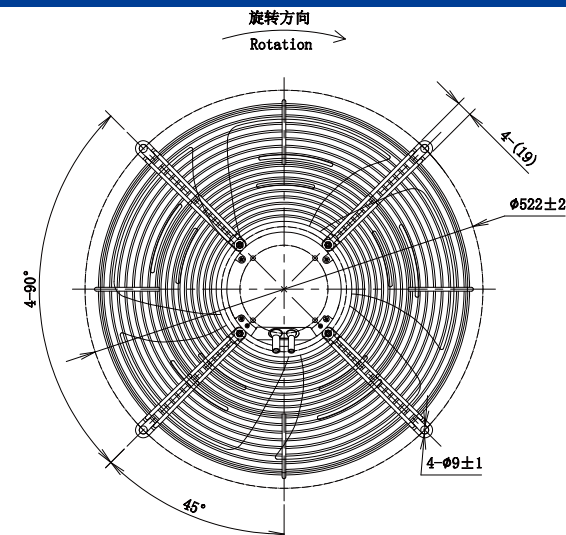
LWAE3G450SS-5MEW-03(Suction)
