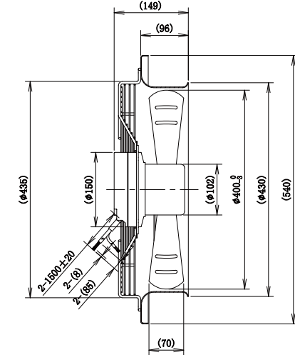
LWAE3G400ST-5MGW-06(Blowing)
