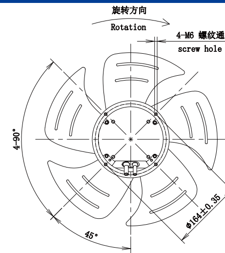
LWAE3G400SS-5MNW-01(Suction)
