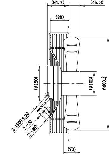
LWAE3G400ST-5MEW-04(Blowing)
