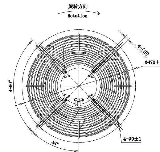
LWAE3G400SS-5MEW-03(Suction)
