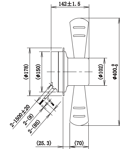
LWAE3G400ST-5MEW-04(Blowing)
