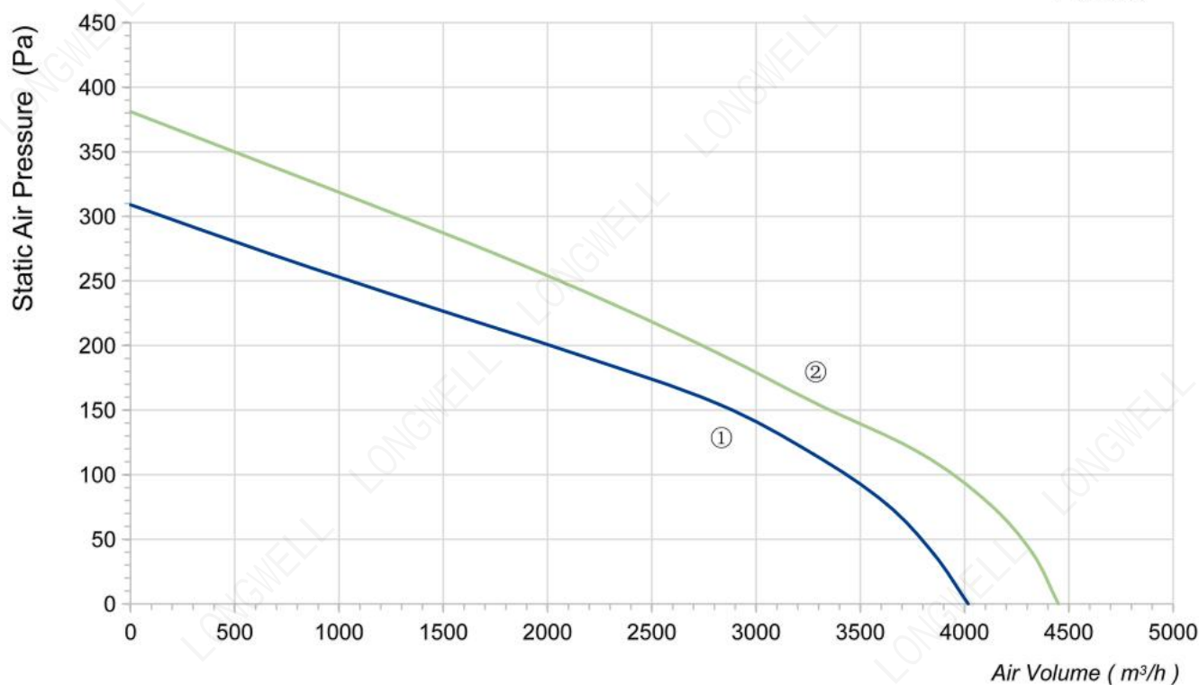
P-Q Curve
