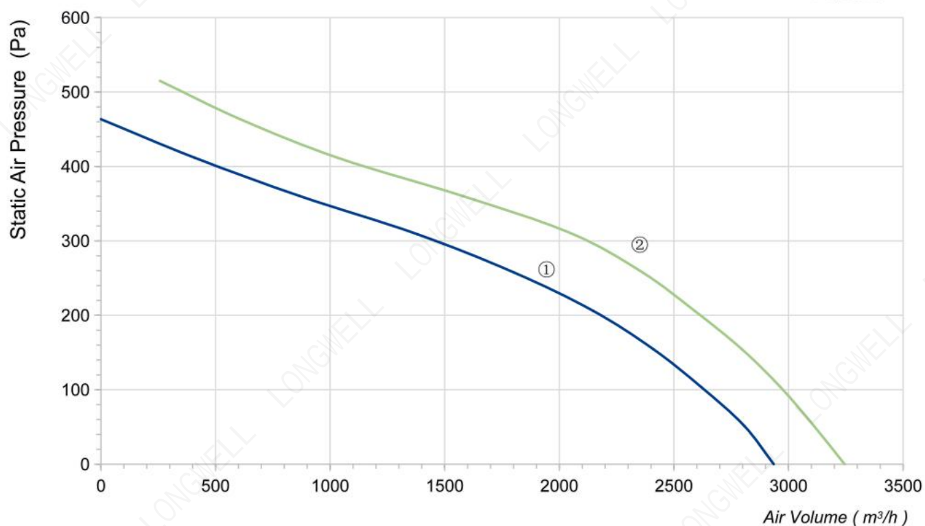
P-Q Curve
