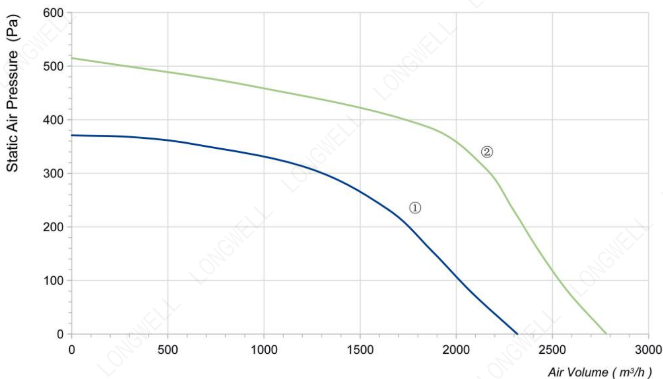
P-Q Curve
