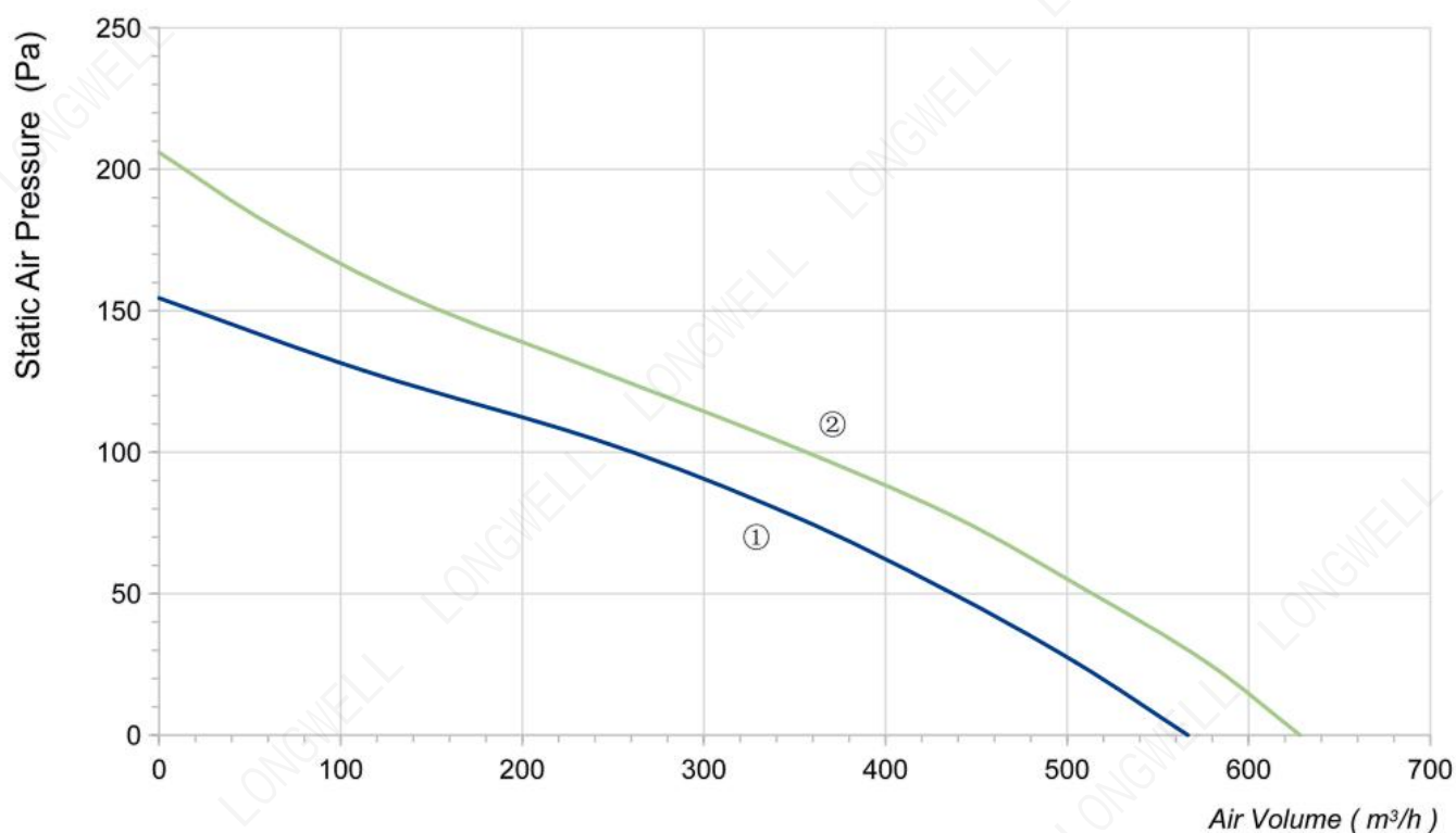
P-Q Curve
