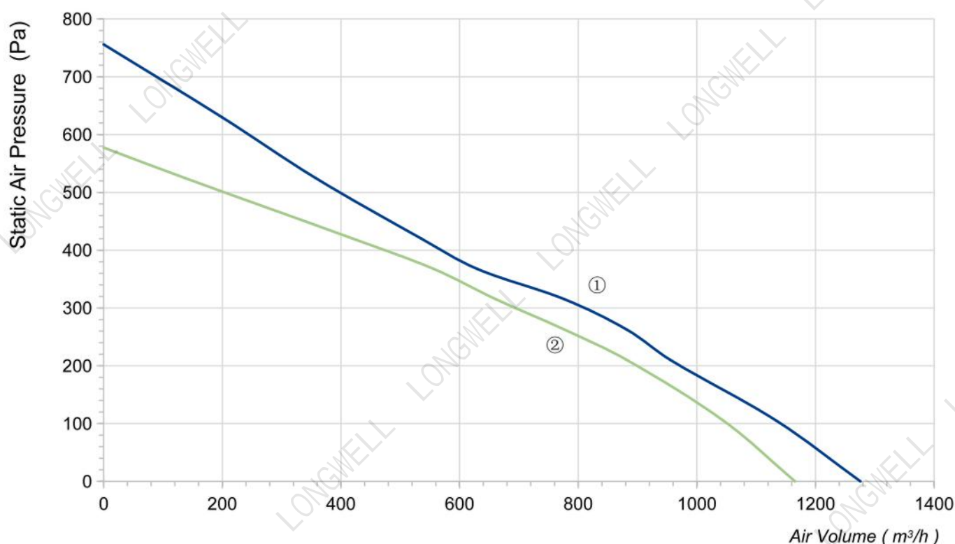
P-Q Curve
