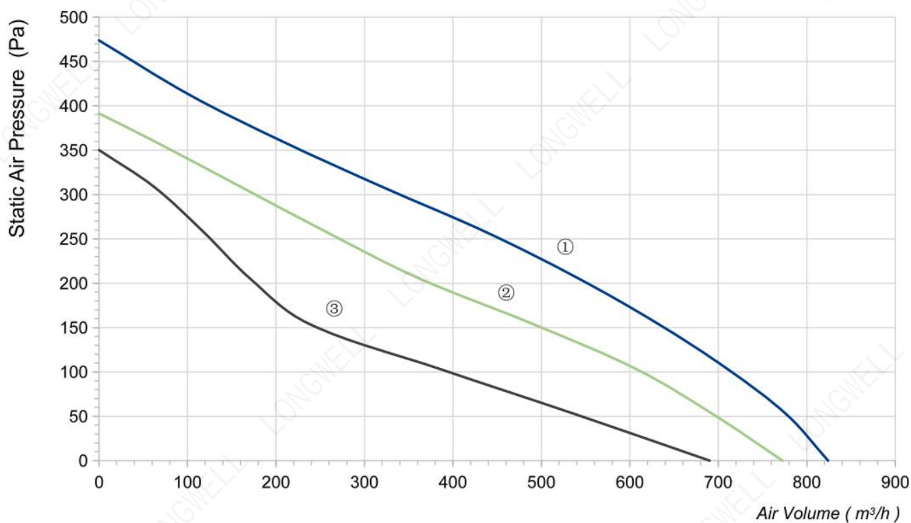
P-Q Curve
