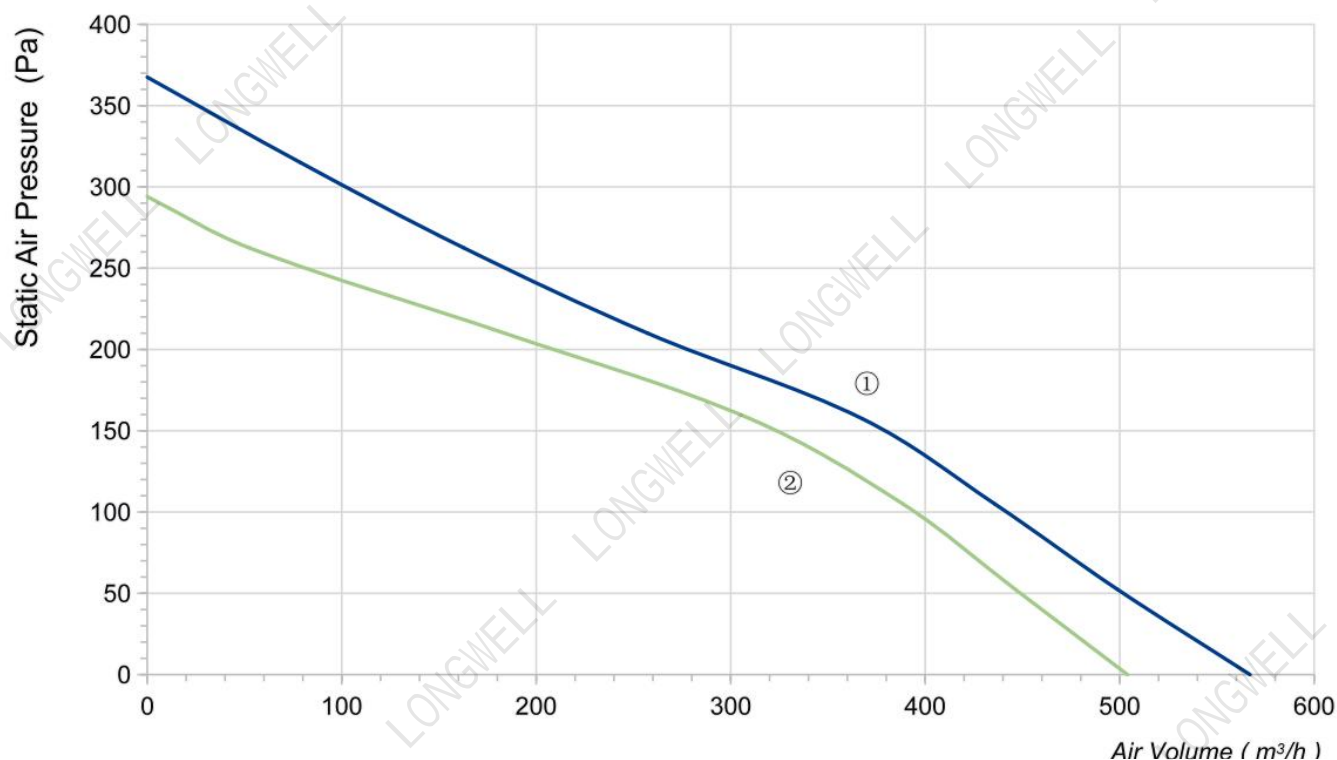
P-Q Curve
