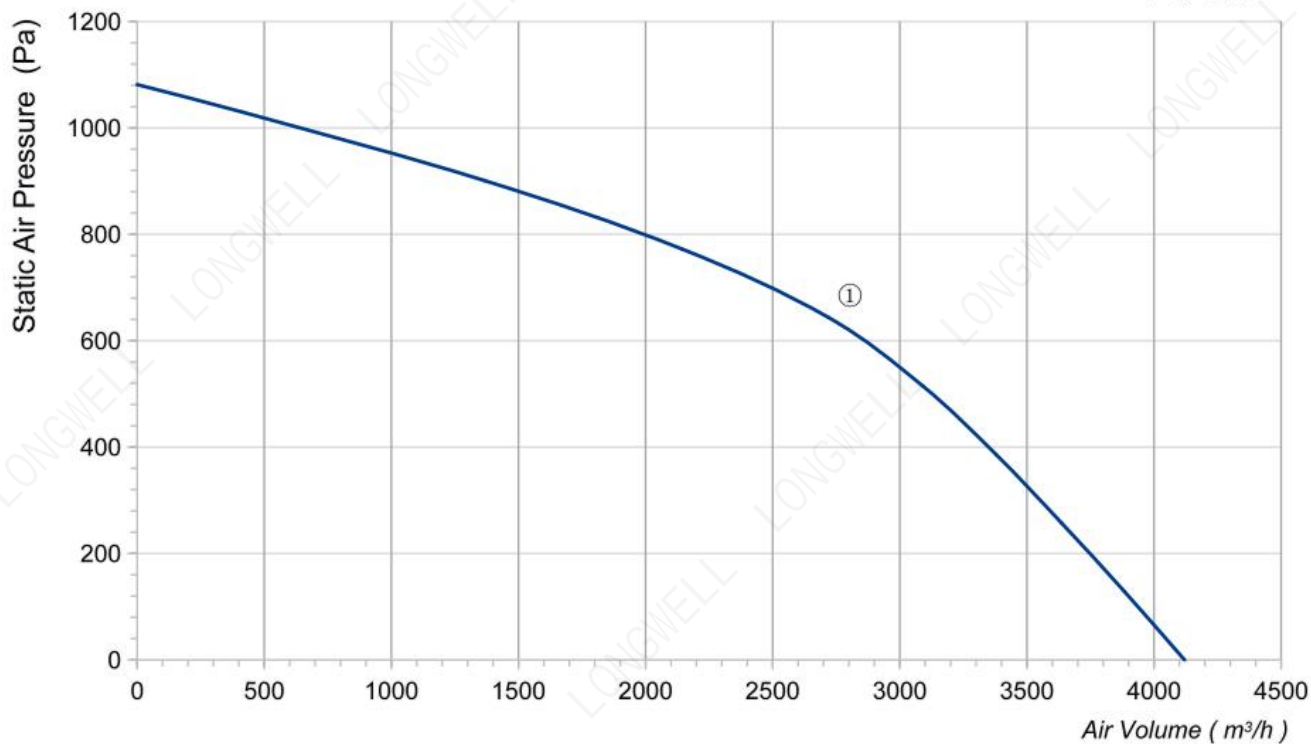
P-Q Curve
