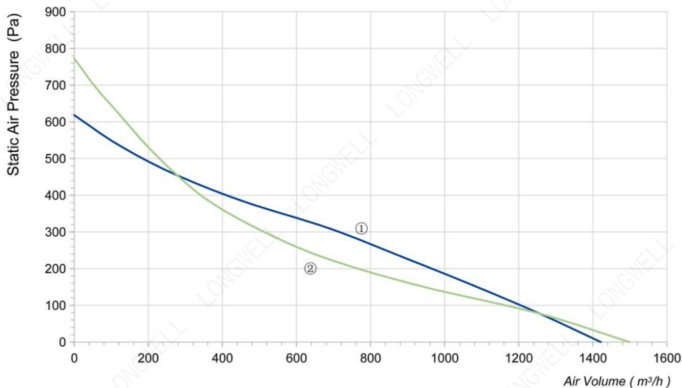
P-Q Curve
