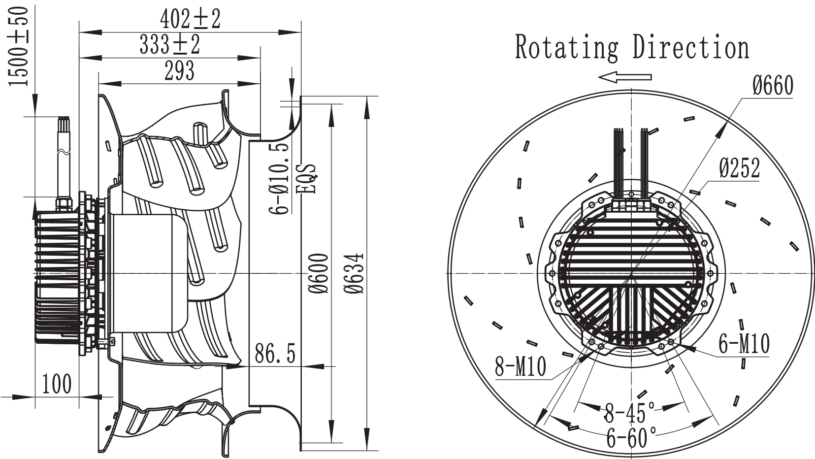
LWBE3G630-188PT-02 (with bracket)
