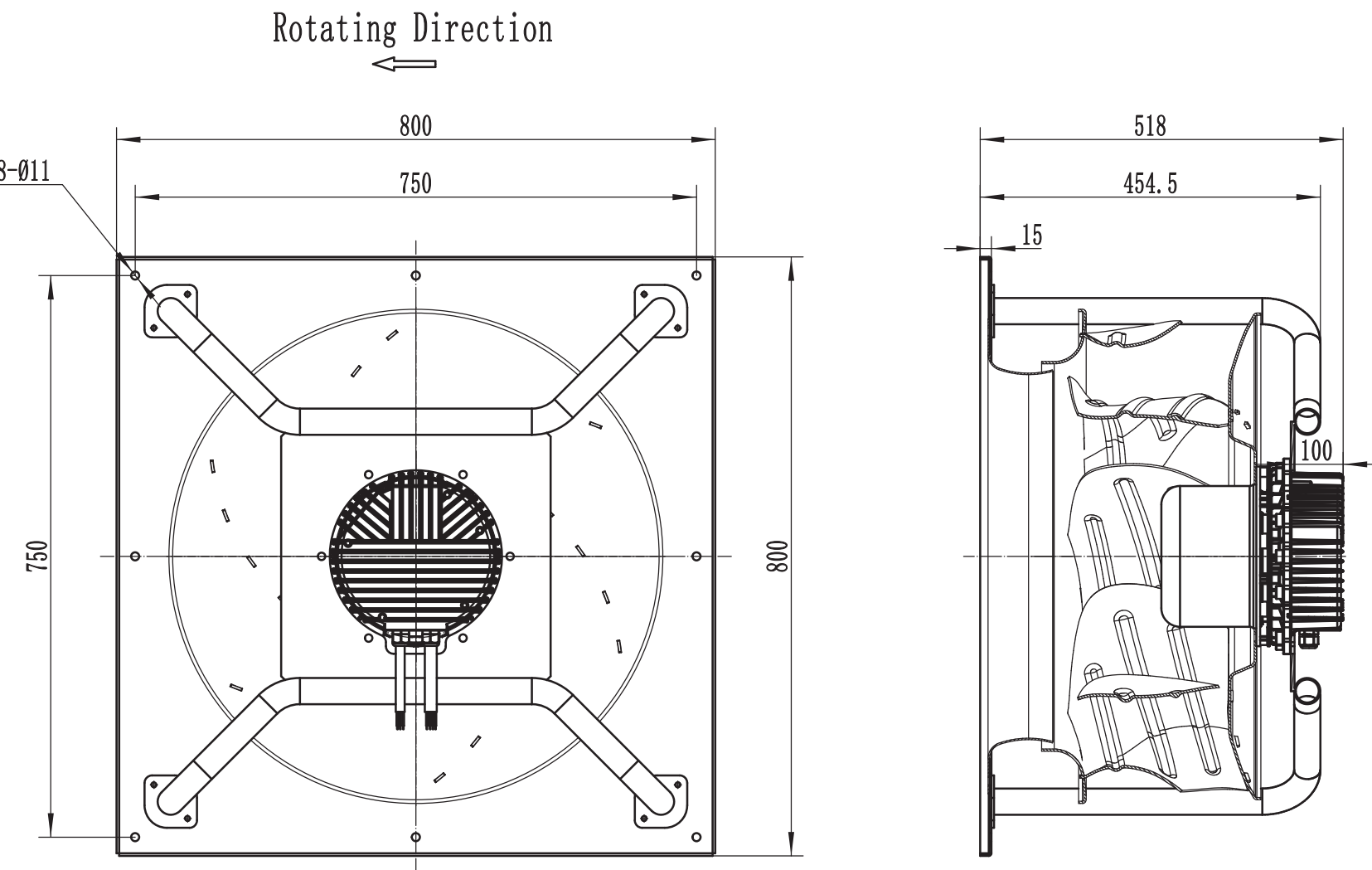
LWBE3G630-188PT-02 (with bracket)
