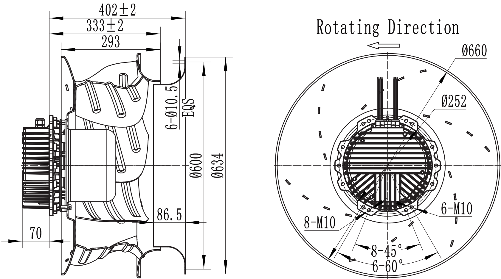
LWBE3G630-188PT-01 (with bracket)
