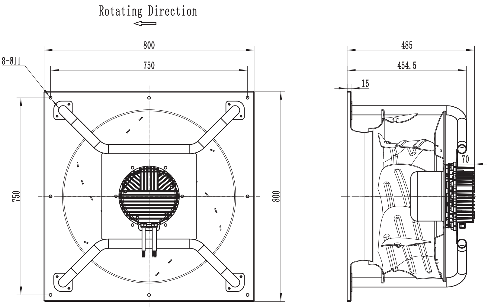
LWBE3G630-188PT-01 (with bracket)
