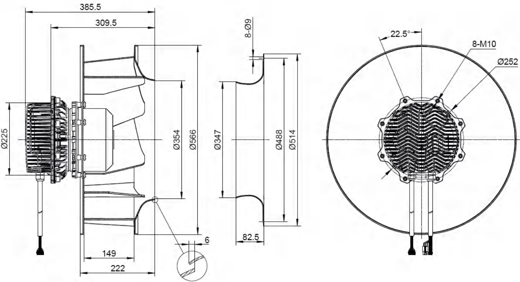
LWBE3G560-218PT-04 (with bracket)
