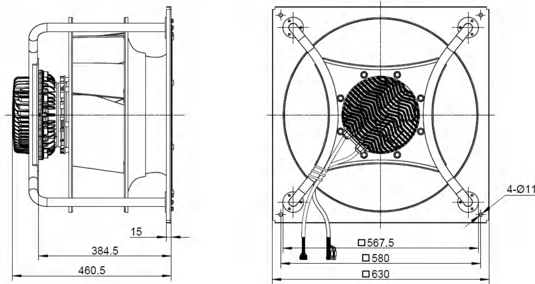
LWBE3G560-218PT-04 (with bracket)
