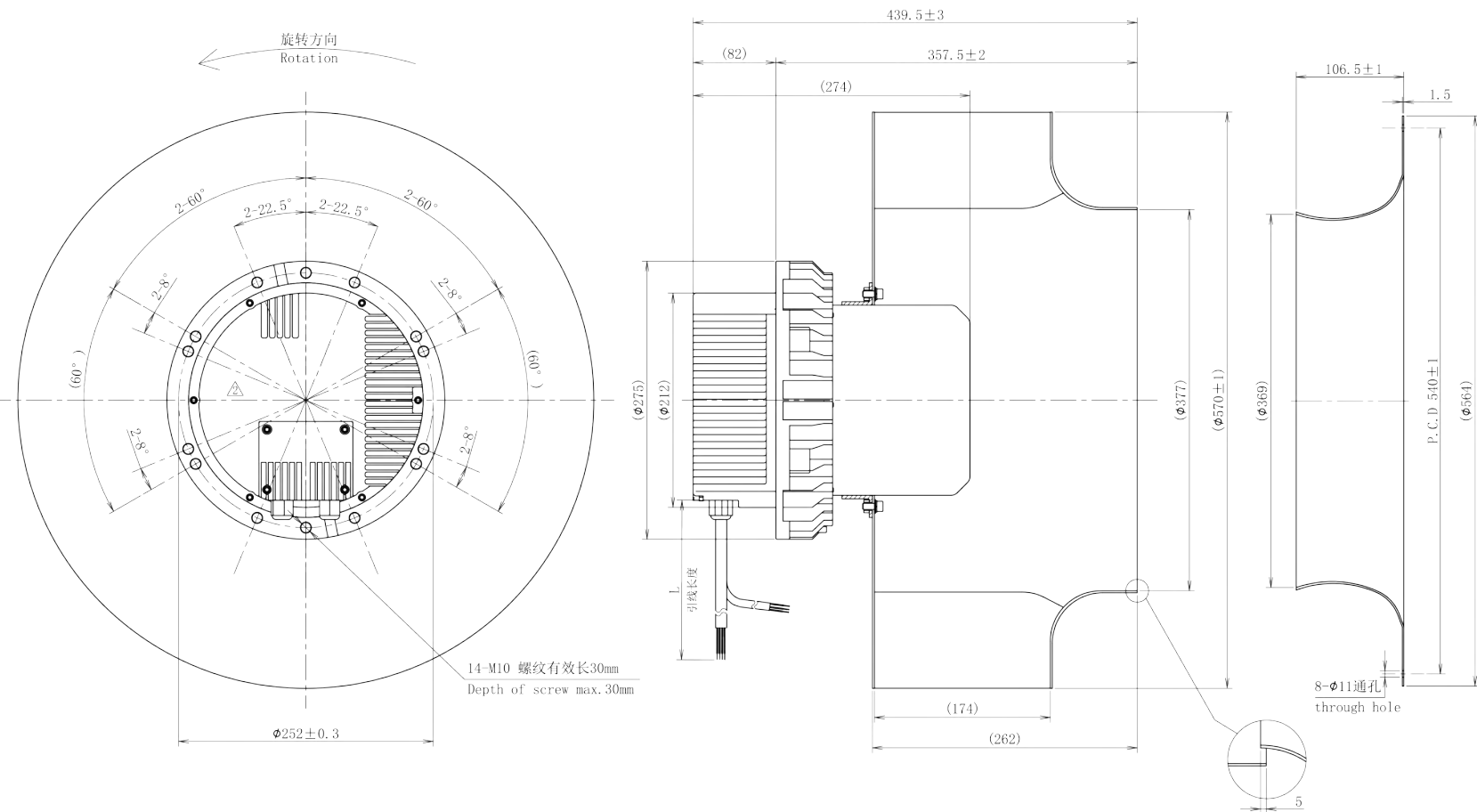
LWBE3G560-188PT-02 (with bracket)
