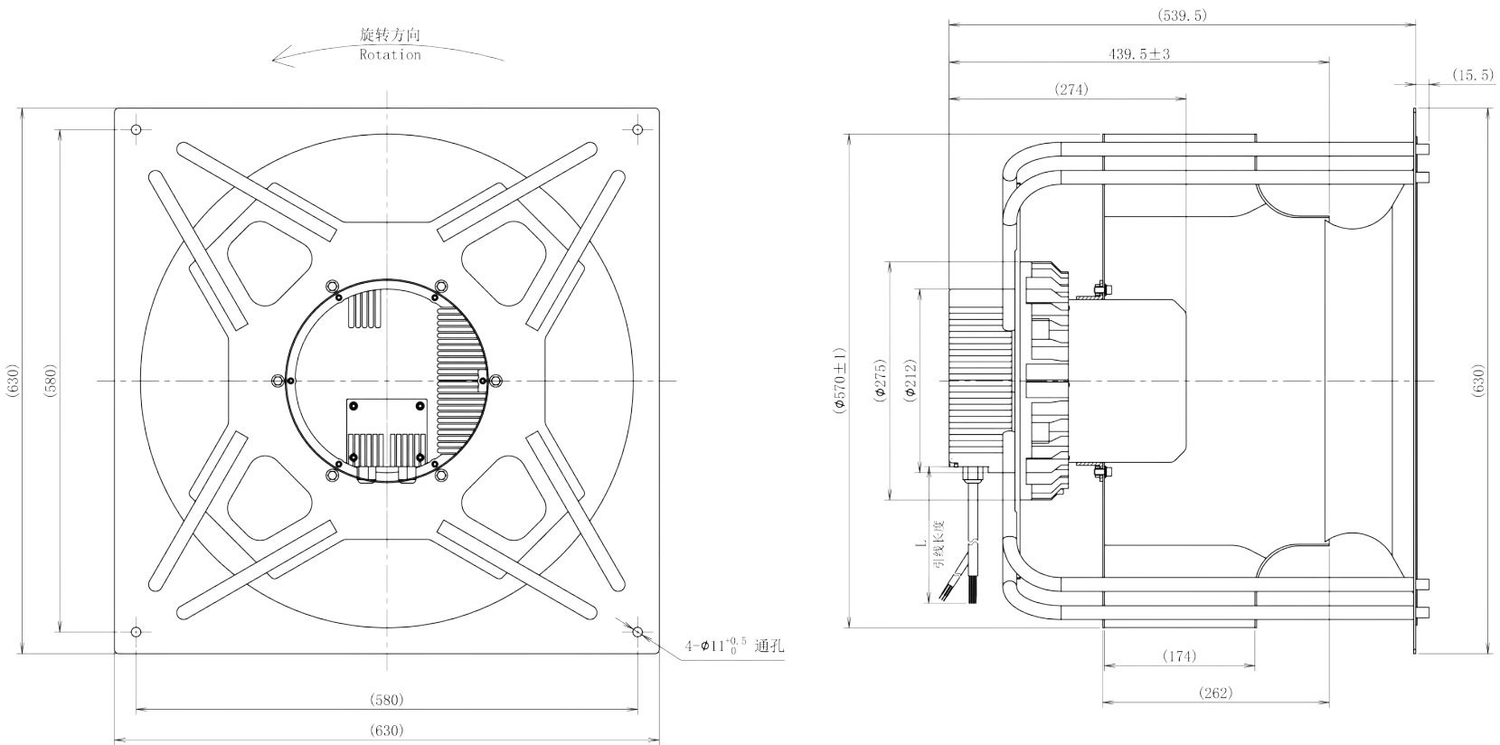
LWBE3G560-188PT-02 (with bracket)
