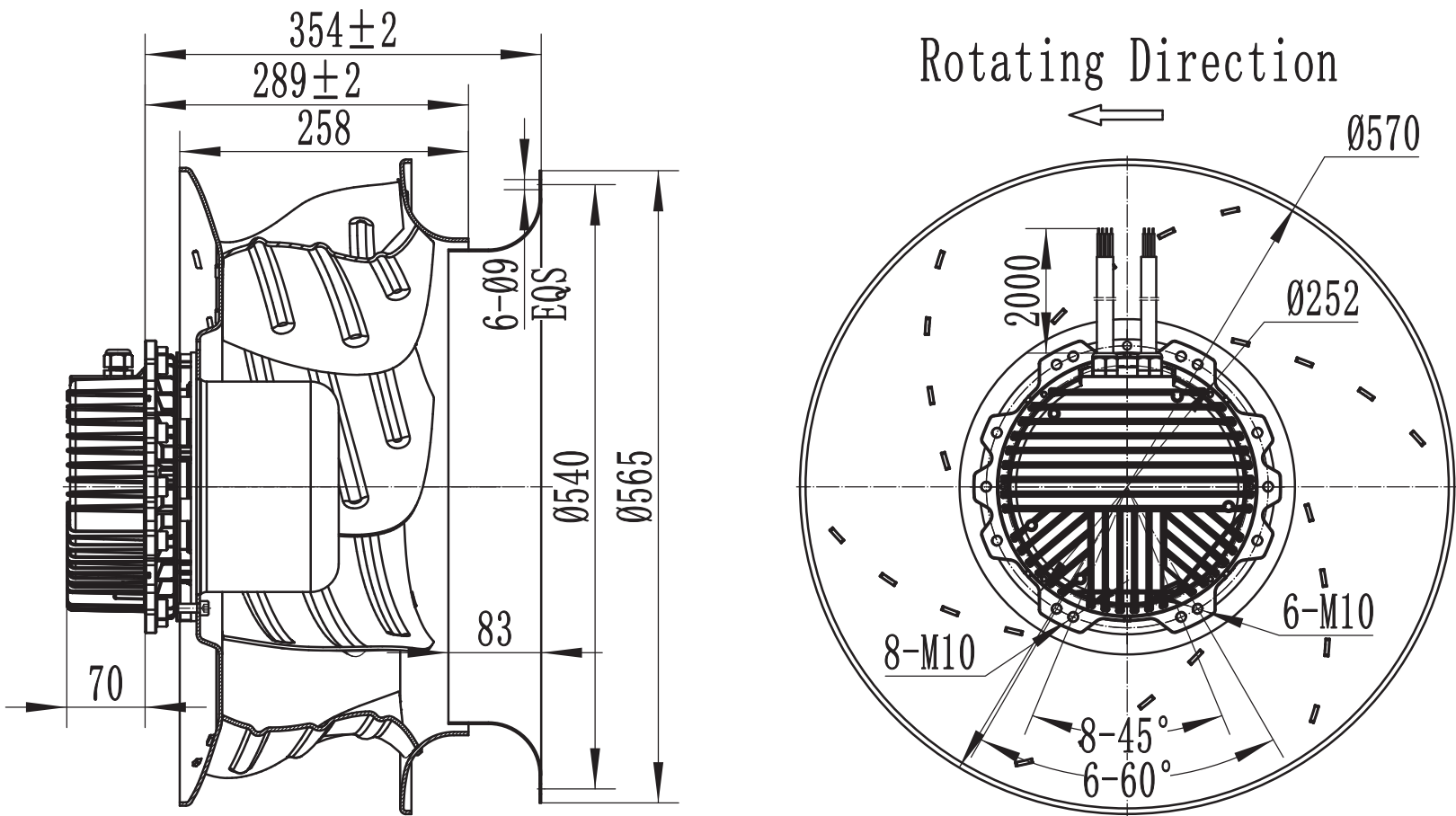
LWBE3G560-188PT-01 (with bracket)
