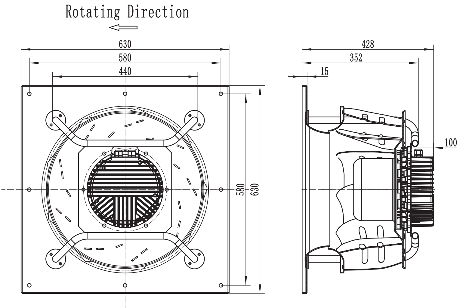
LWBE3G500-188PT-05 (with bracket)
