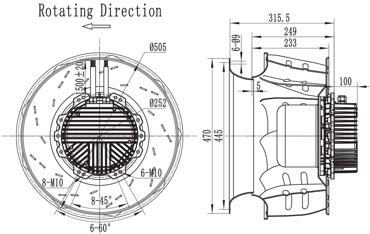
LWBE3G500-188PT-05 (with bracket)
