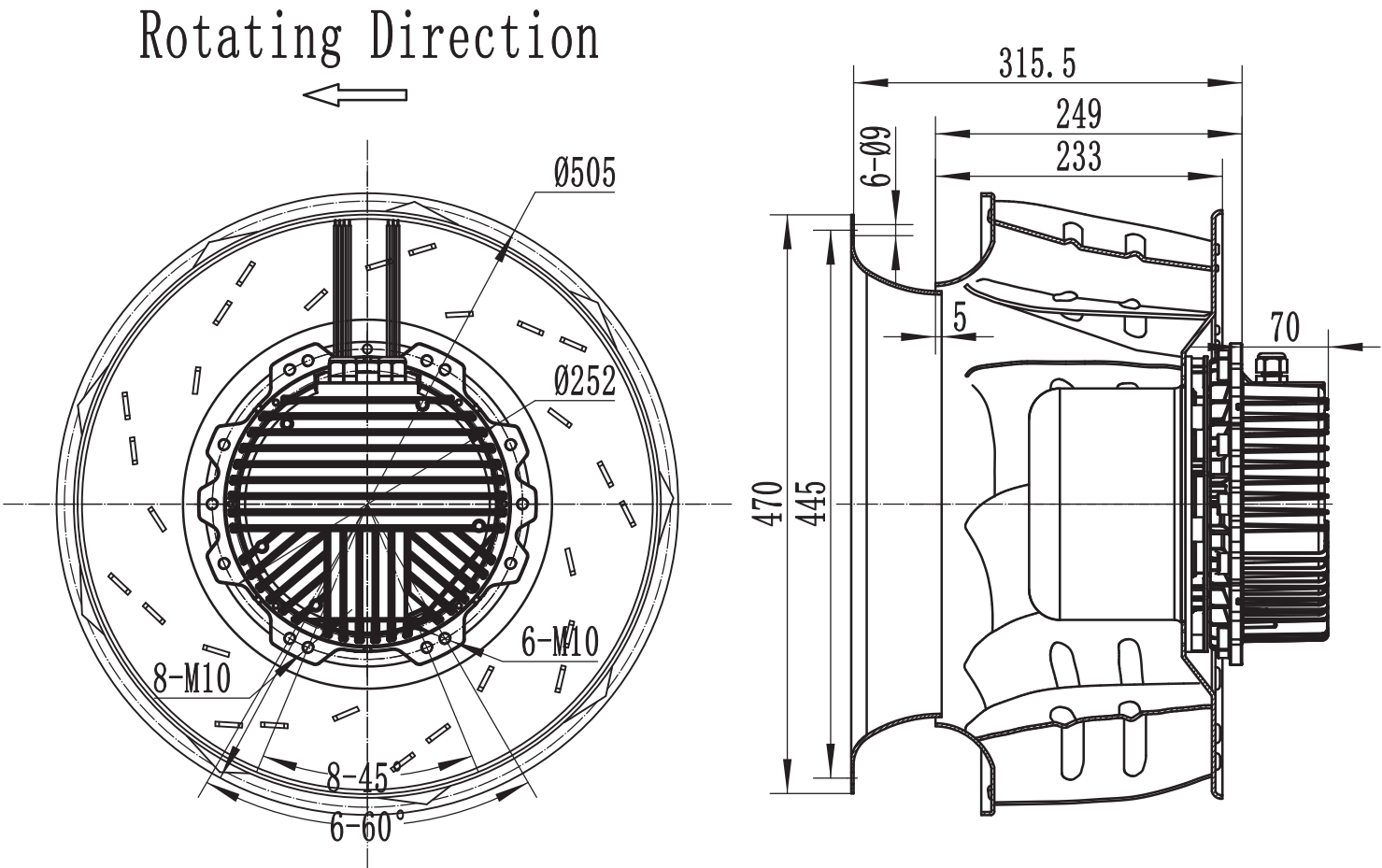
LWBE3G500-188PT-02 (with bracket)
