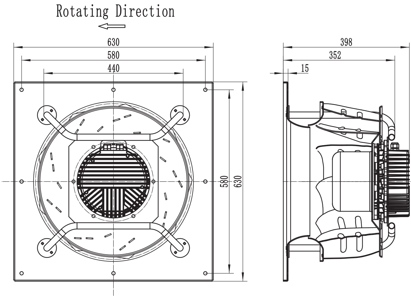
LWBE3G500-188PT-02 (with bracket)
