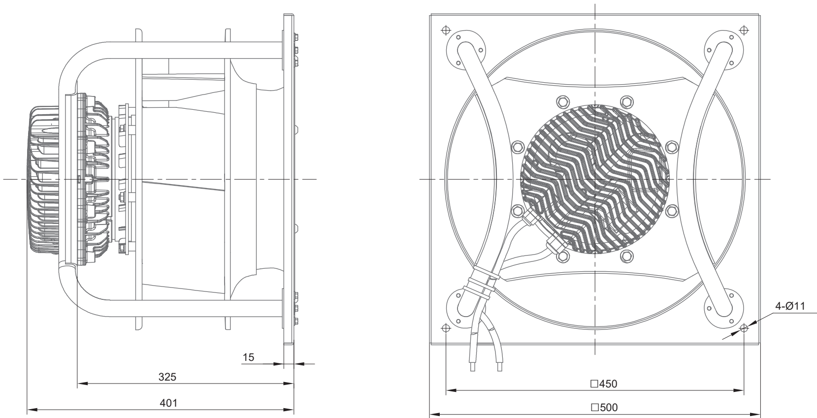
LWBE3G450-188PT-05 (with bracket)
