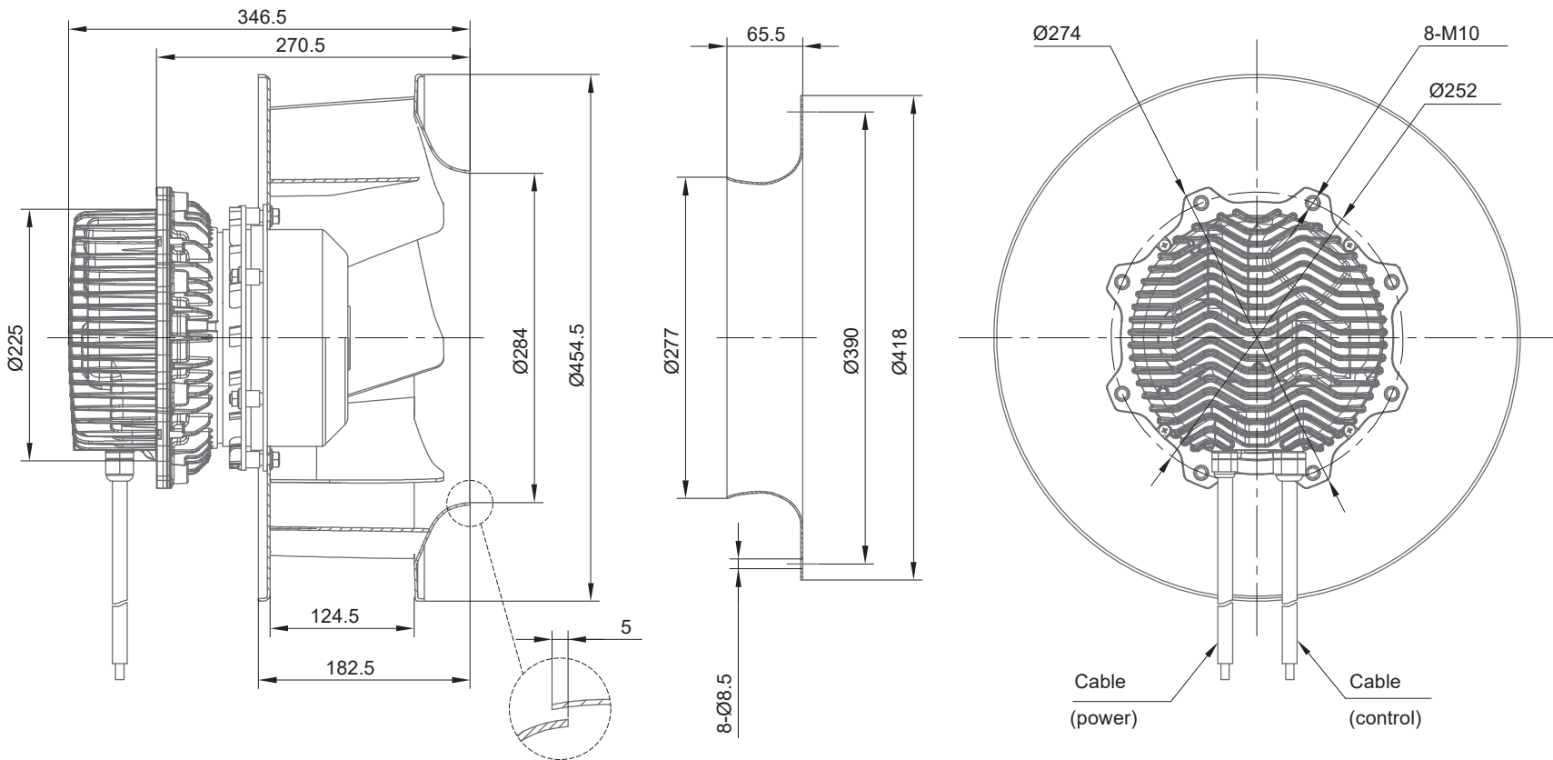
LWBE3G450-188NT-009 (without bracket)
