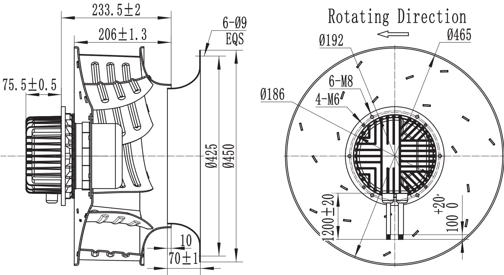
LWBE3G450-138NT-008 (without bracket)
