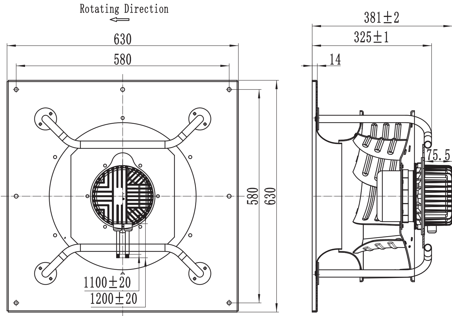
LWBE3G450-138PT-04 (with bracket)
