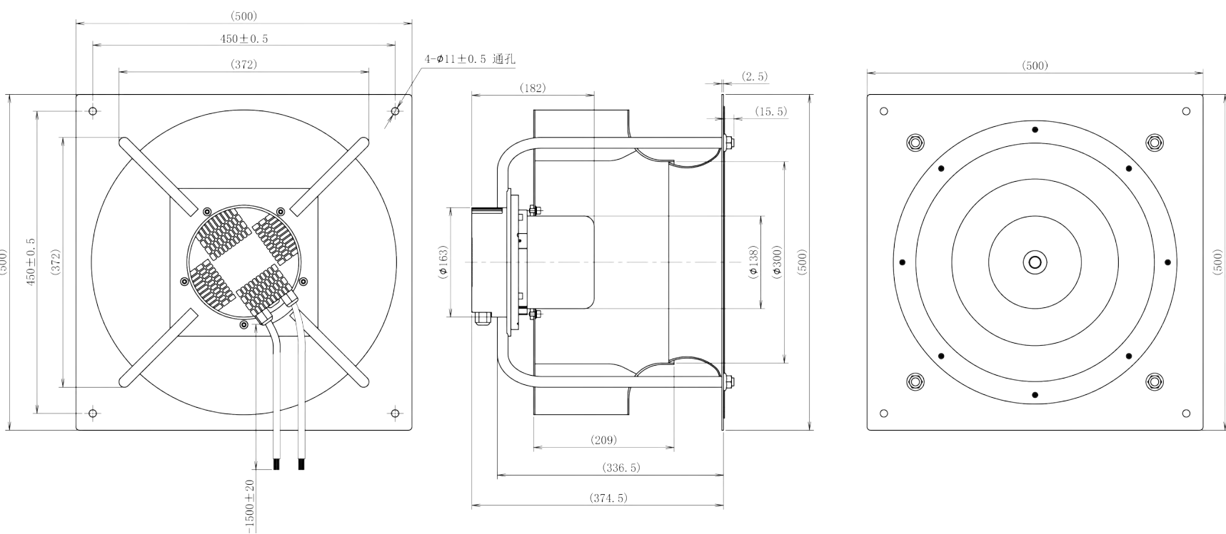
LWBE3G450-138PT-02 (with bracket)
