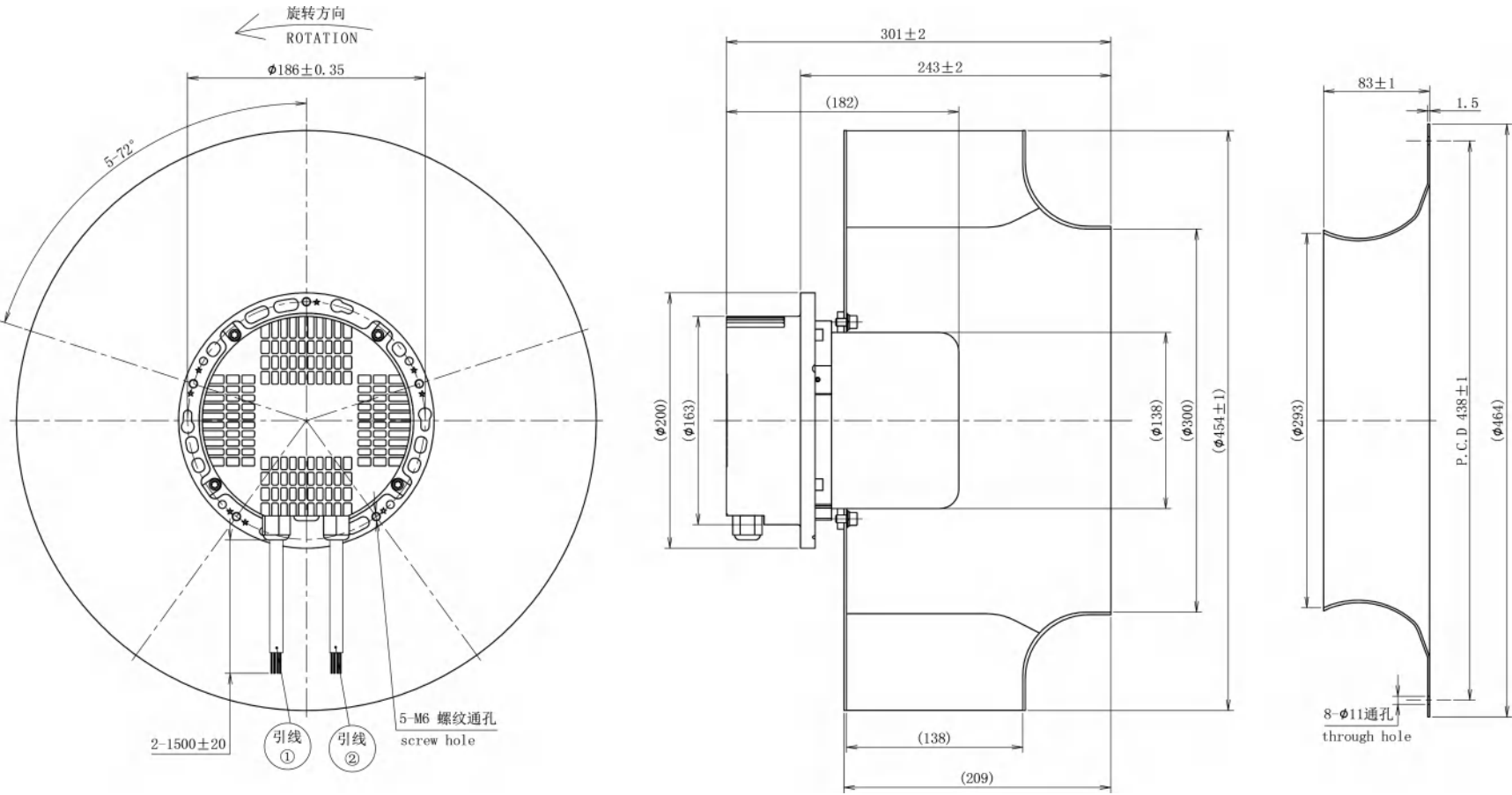
LWBE3G450-138PT-02 (with bracket)
