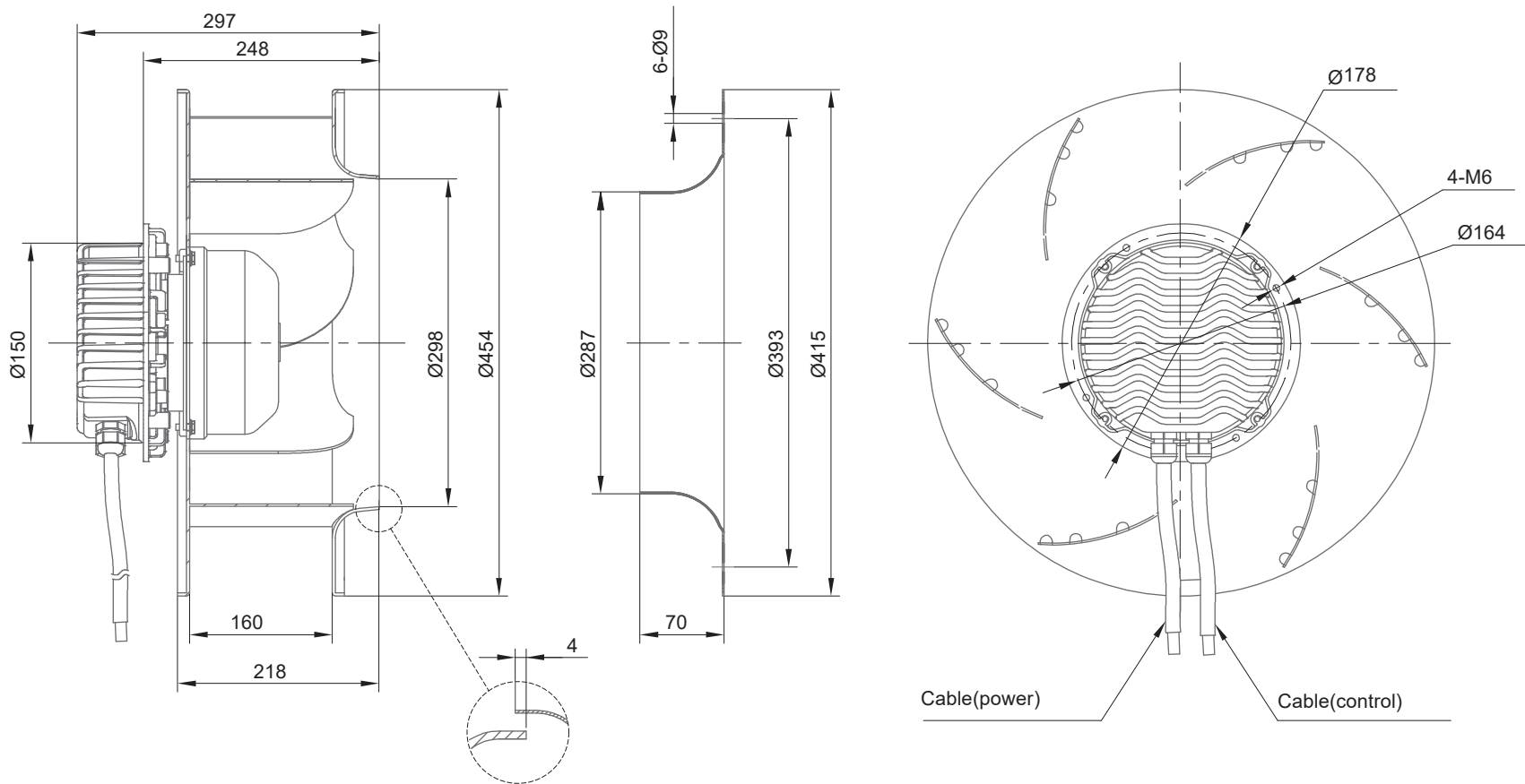
LWBE3G450-102PS-01 (with bracket)
