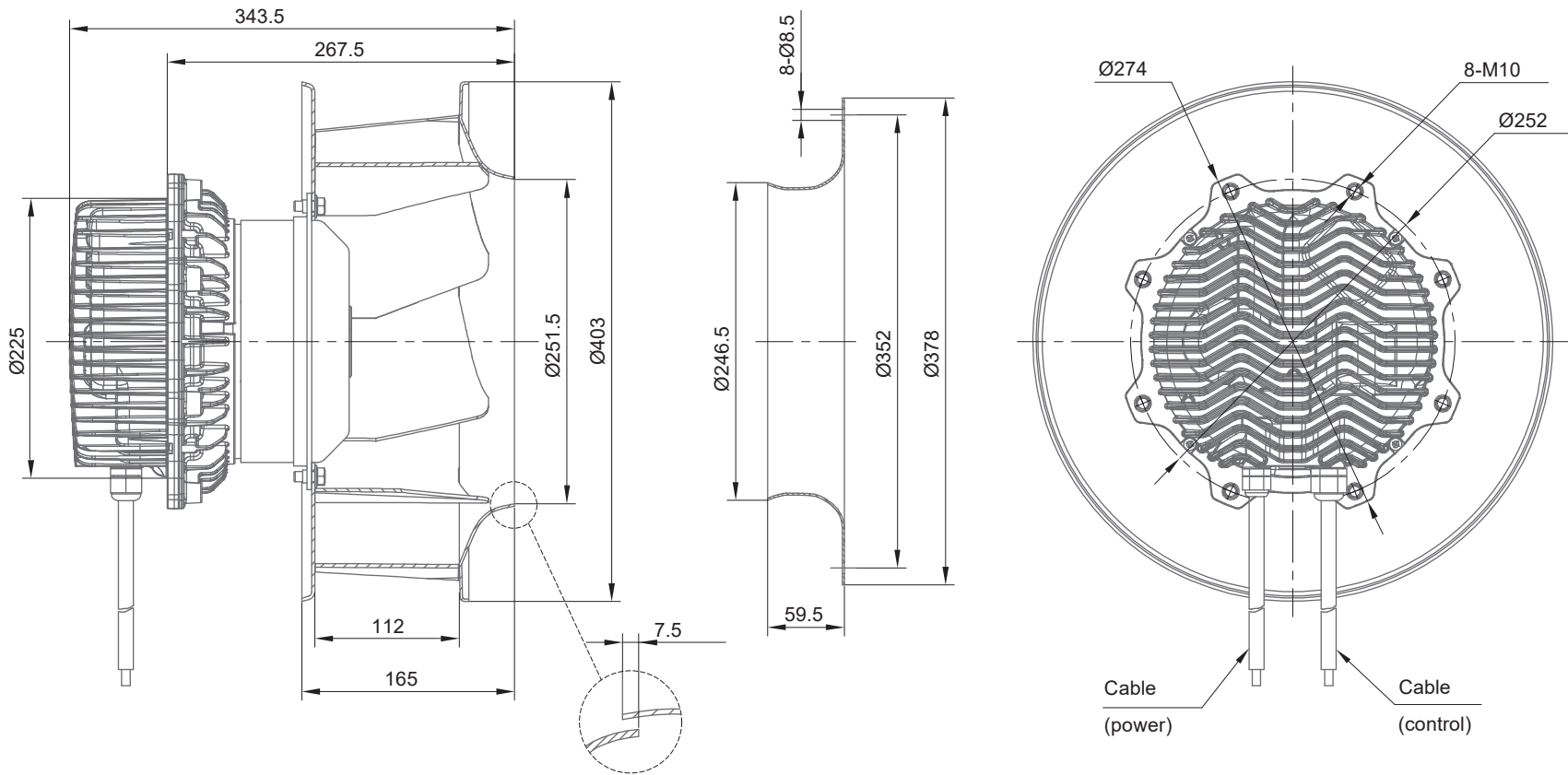
LWBE3G400-188PT-05 (with bracket)
