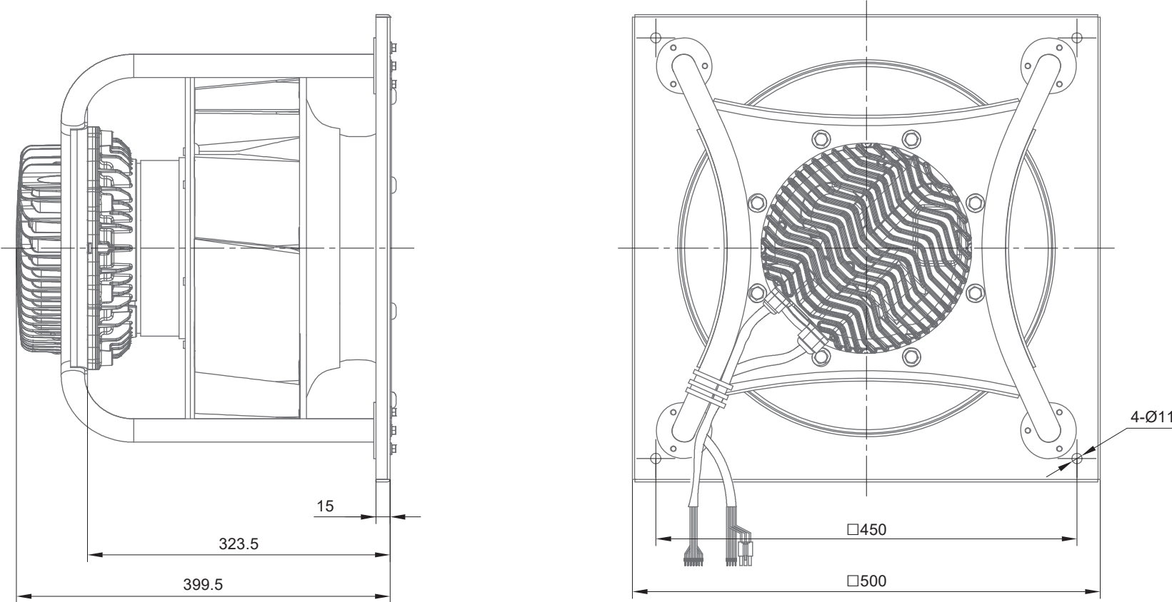
LWBE3G400-188PT-05 (with bracket)
