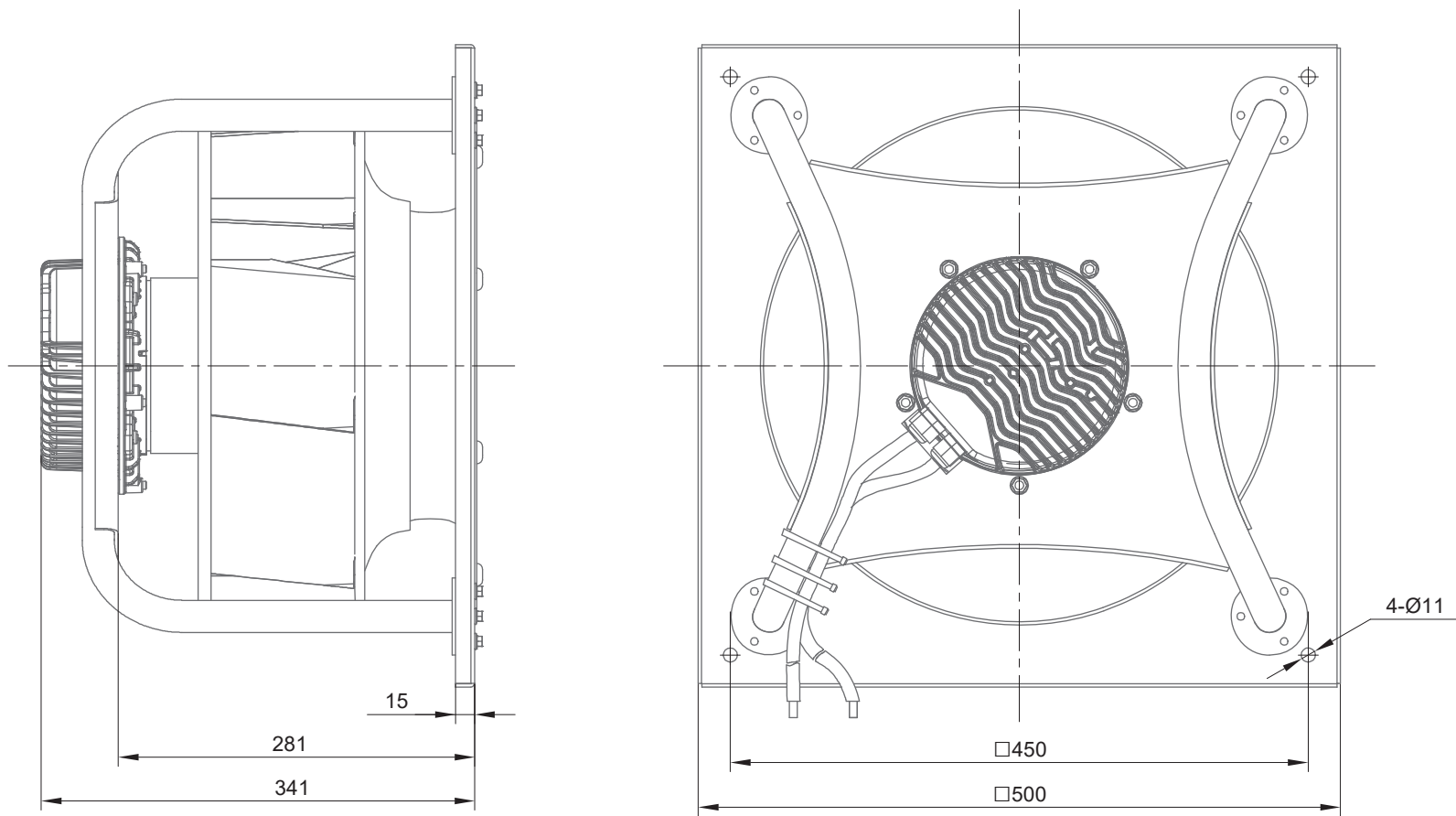
LWBE3G400-138PT-03 (with bracket)
