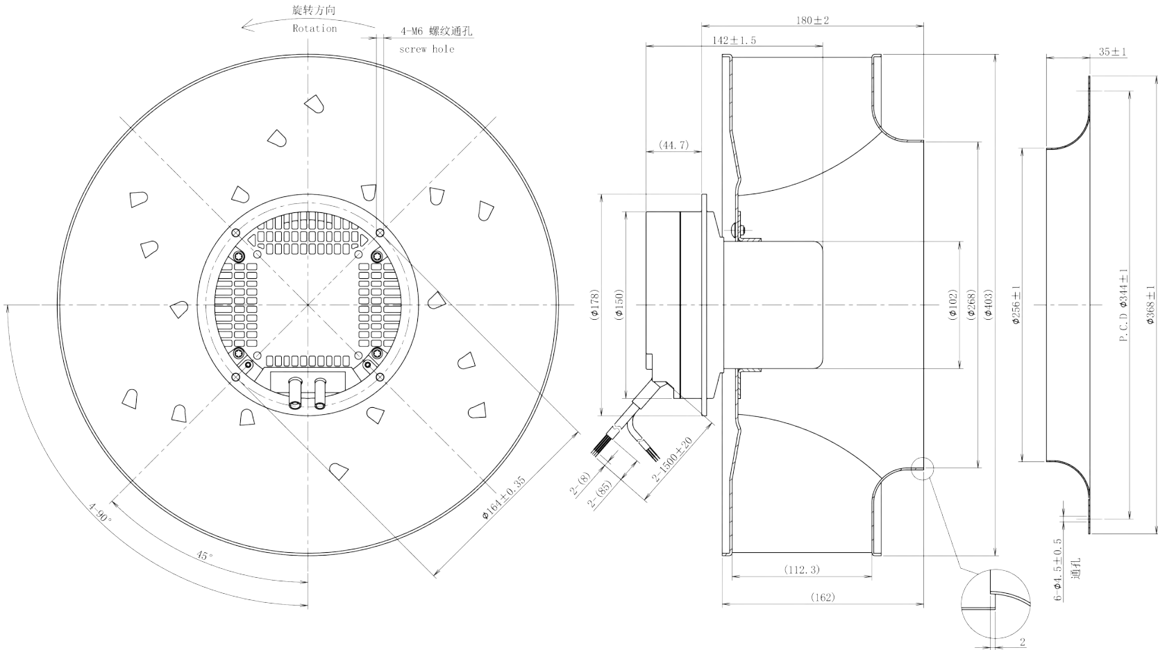
LWBE3G400-102PS-01 (with bracket)
