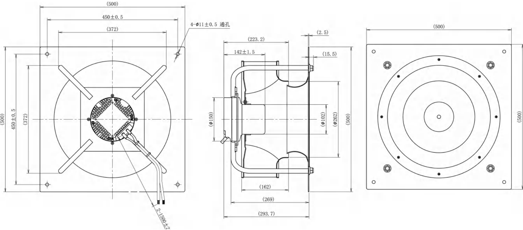
LWBE3G400-102PS-01 (with bracket)
