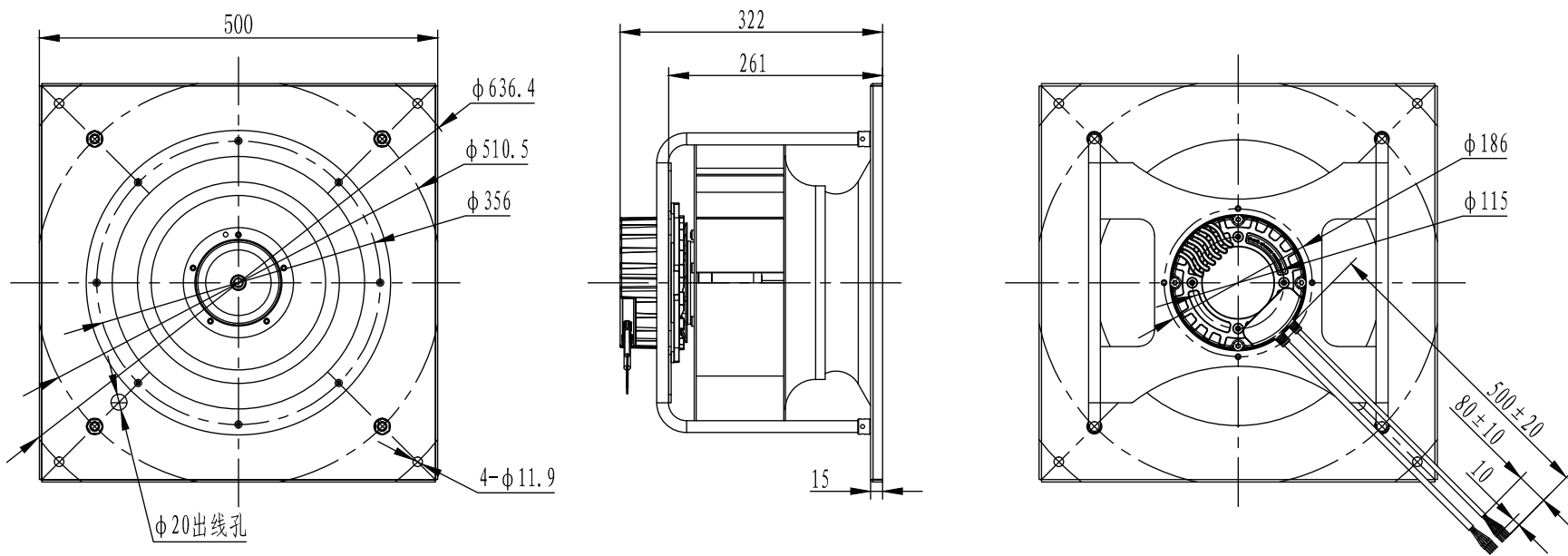
LWBE3G355-102PS-03 (with bracket)
