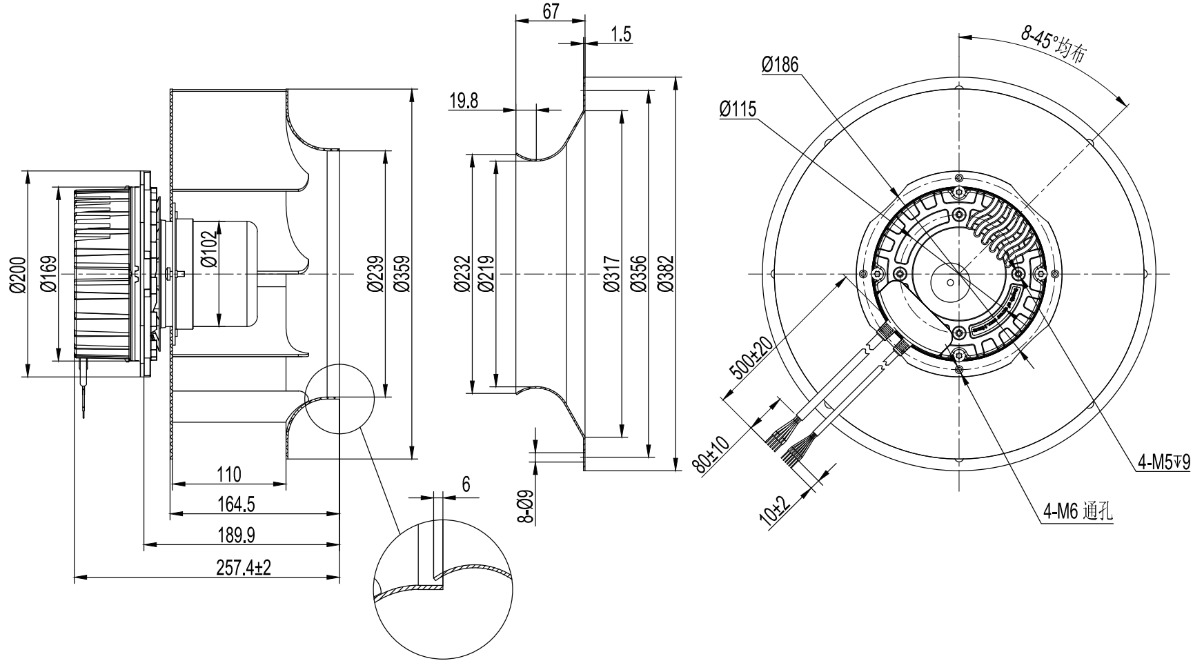
LWBE3G355-102PS-03 (with bracket)
