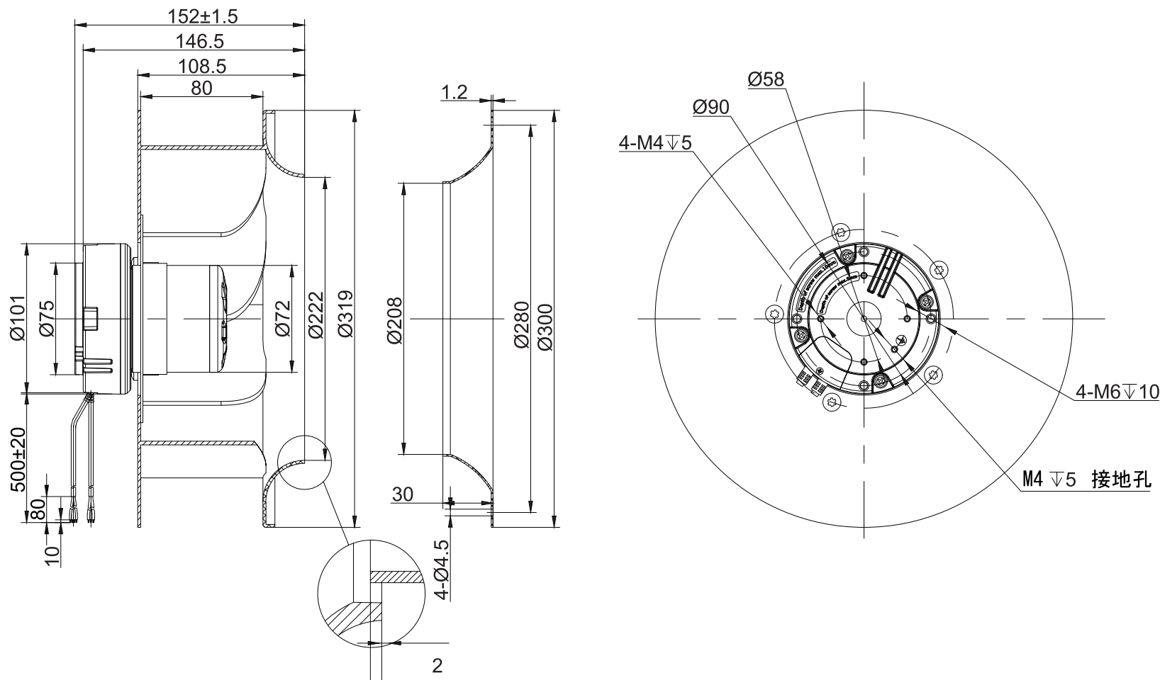
LWBE3G310-72PS-01 (with bracket)
