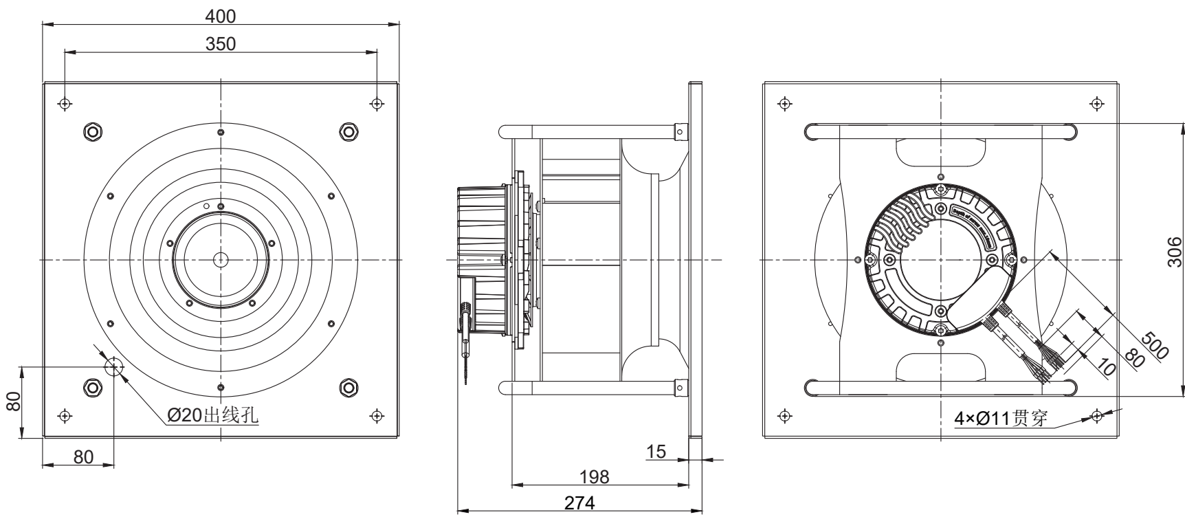
LWBE3G280-102PS-04 (with bracket)
