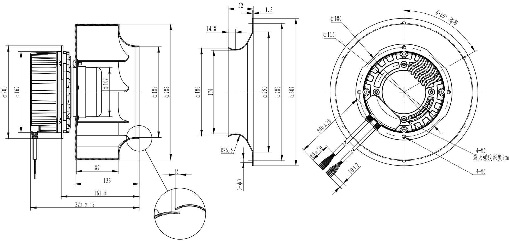
LWBE3G280-102PS-04 (with bracket)
