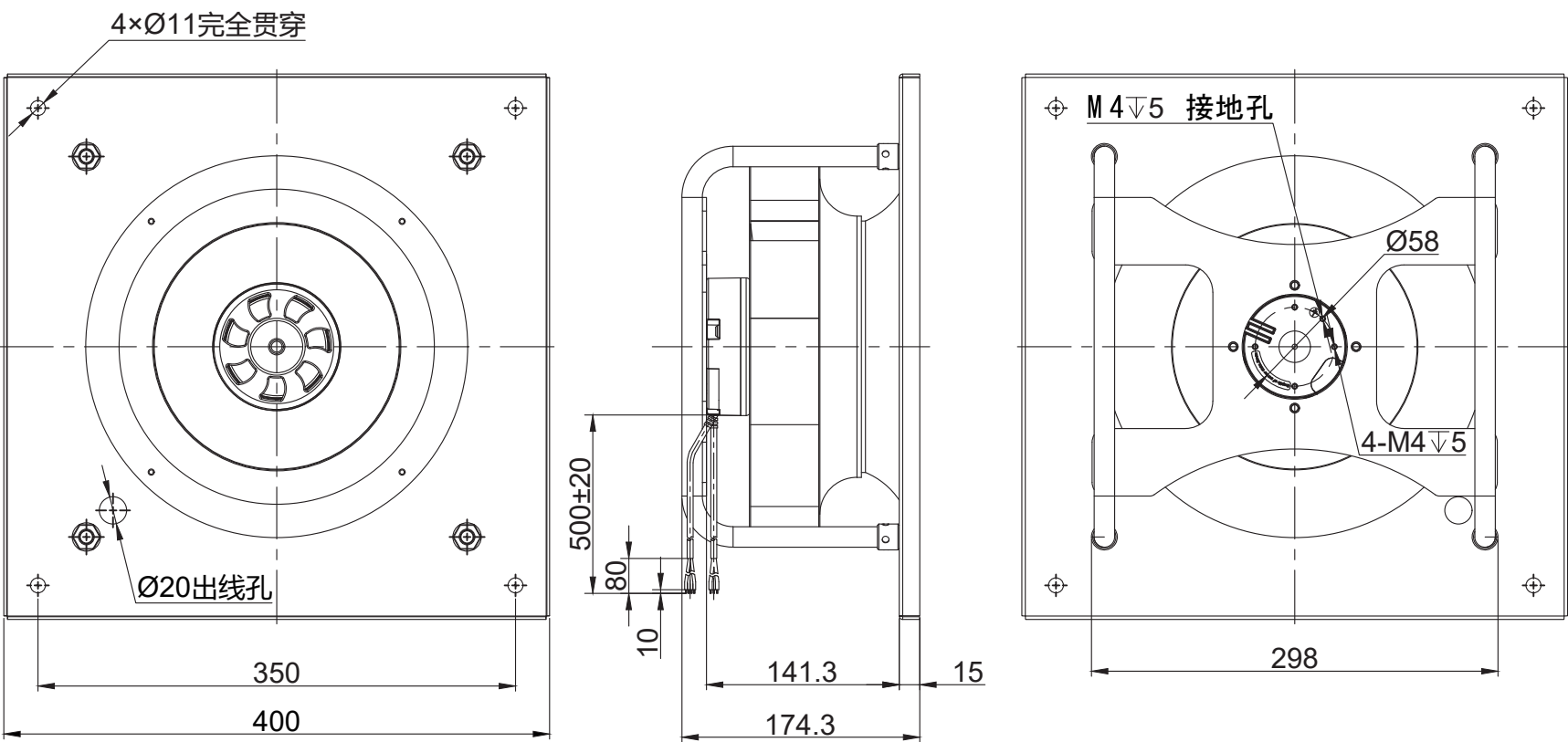
LWBE3G280-92PS-03 (with bracket)
