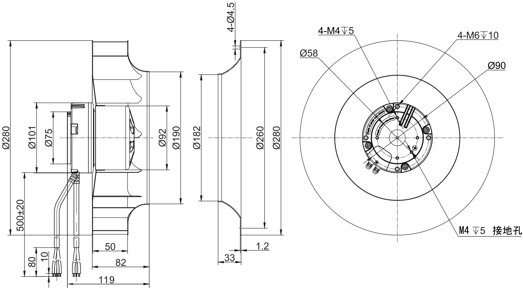
LWBE3G280-92PS-03 (with bracket)
