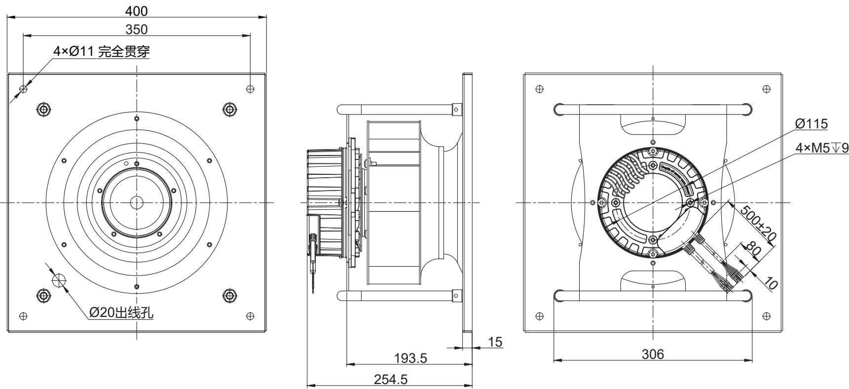
LWBE3G250-102PS-07(with bracket)
