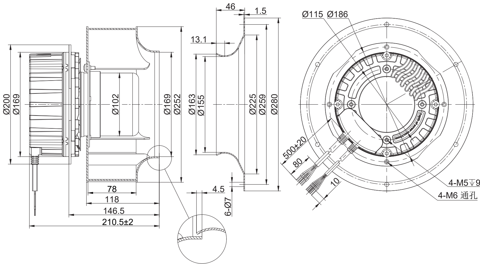
LWBE3G250-102PS-07(with bracket)
