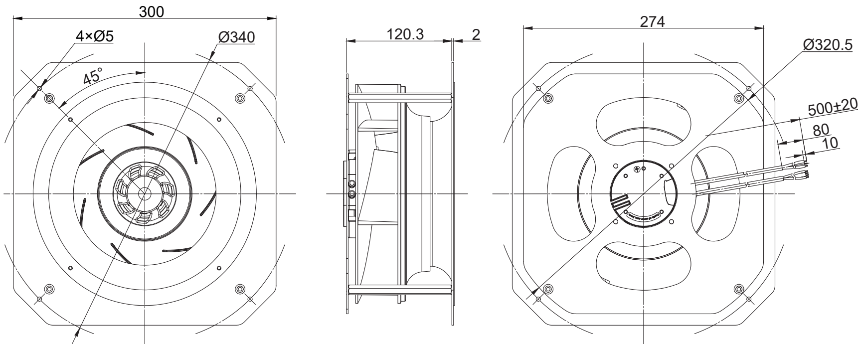
LWBE3G250-72PS-04 (with bracket)
