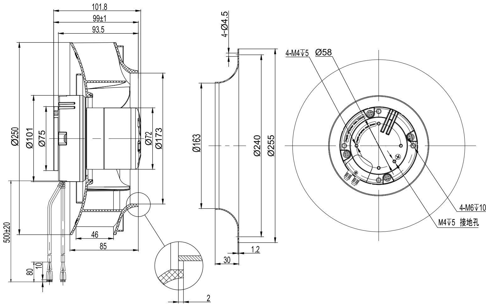
LWBE3G250-72PS-04 (with bracket)
