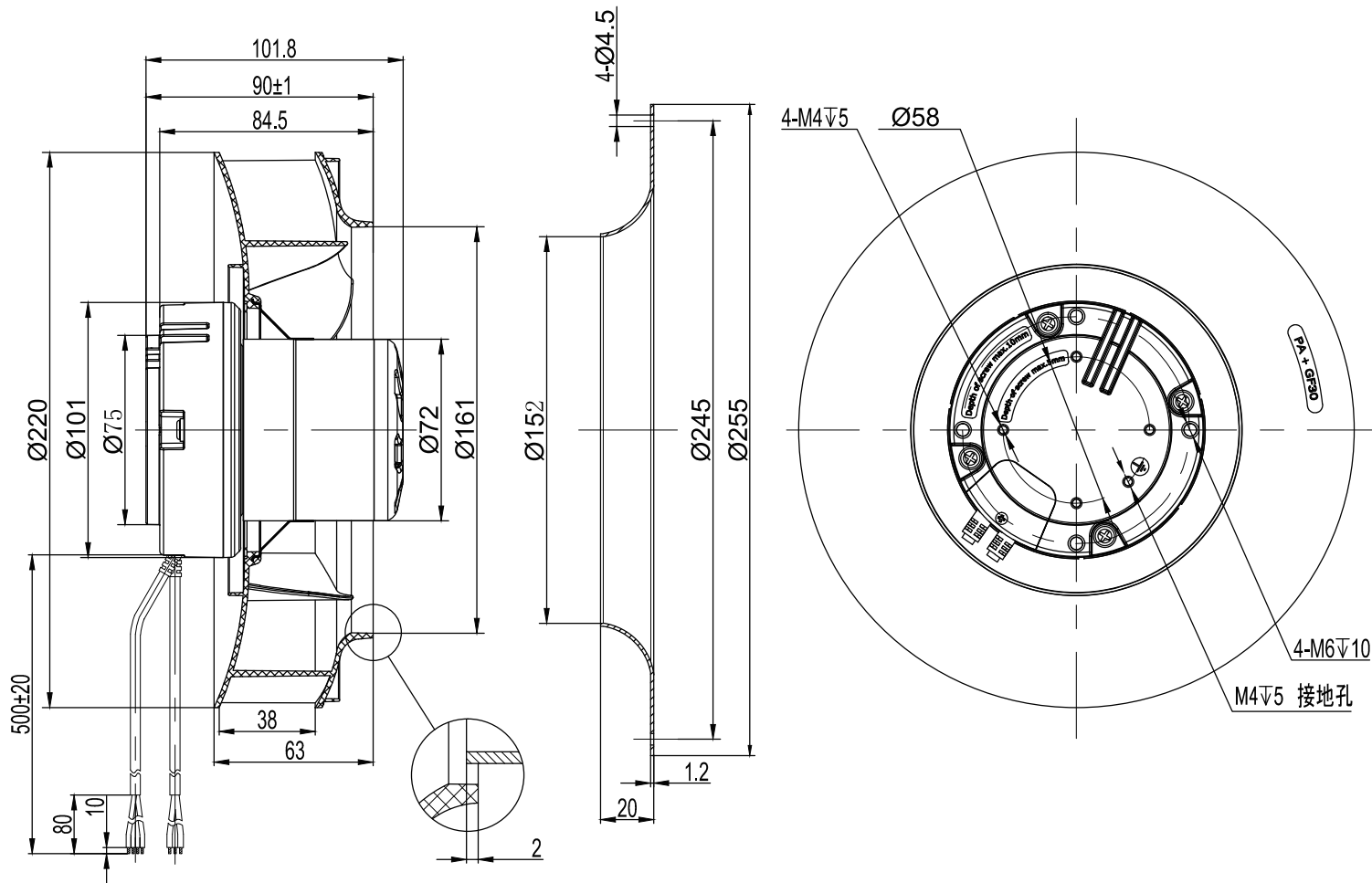
LWBE3G220-72PS-03 (with bracket)
