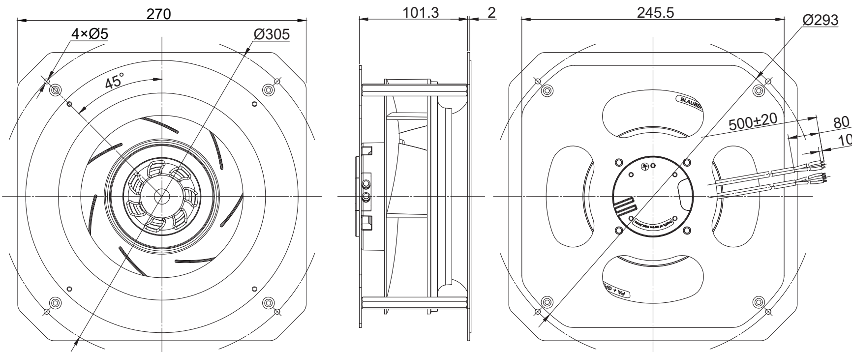
LWBE3G220-72PS-03 (with bracket)
