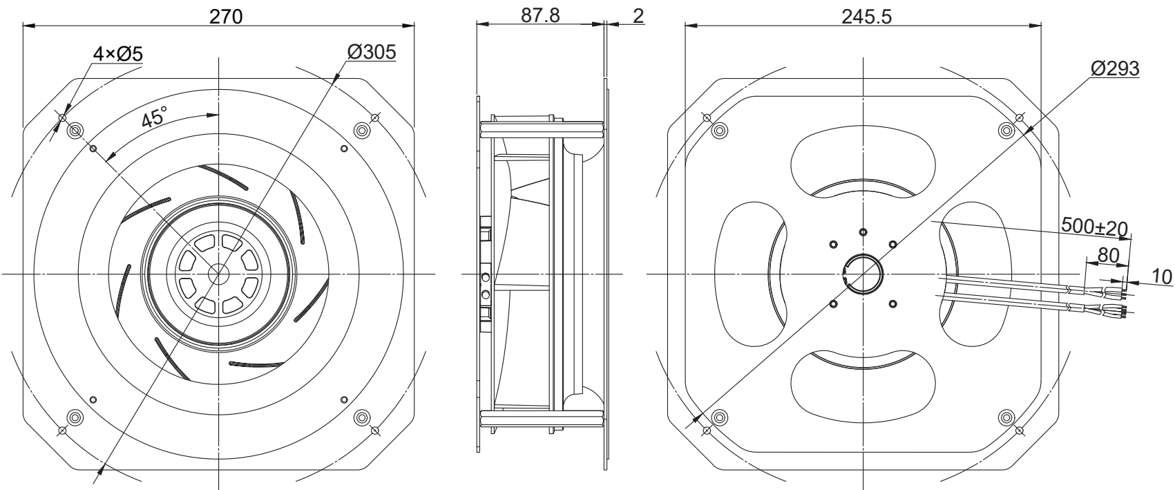
LWBE3G220-72PS-01 (with bracket)
