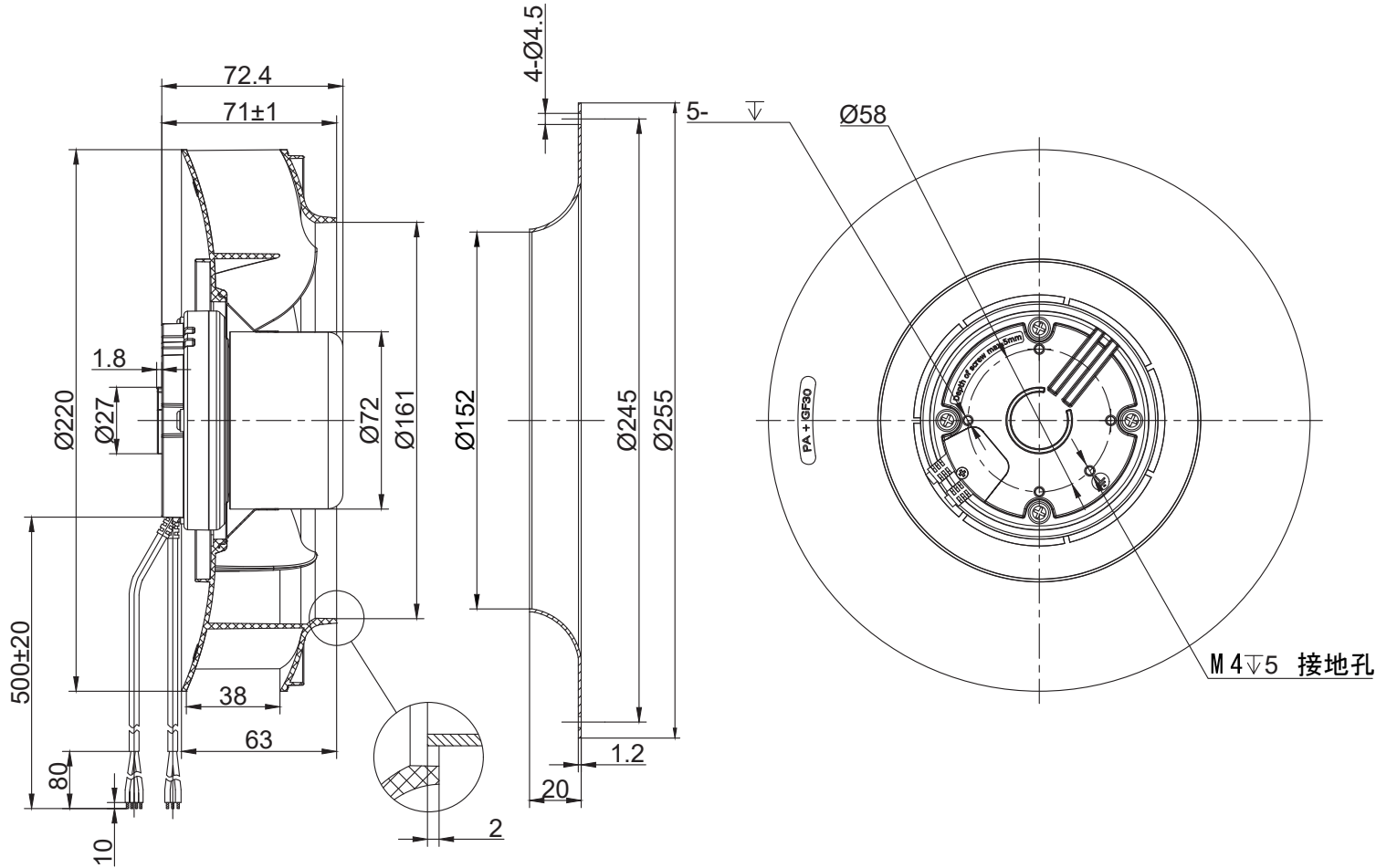
LWBE3G220-72PS-01 (with bracket)
