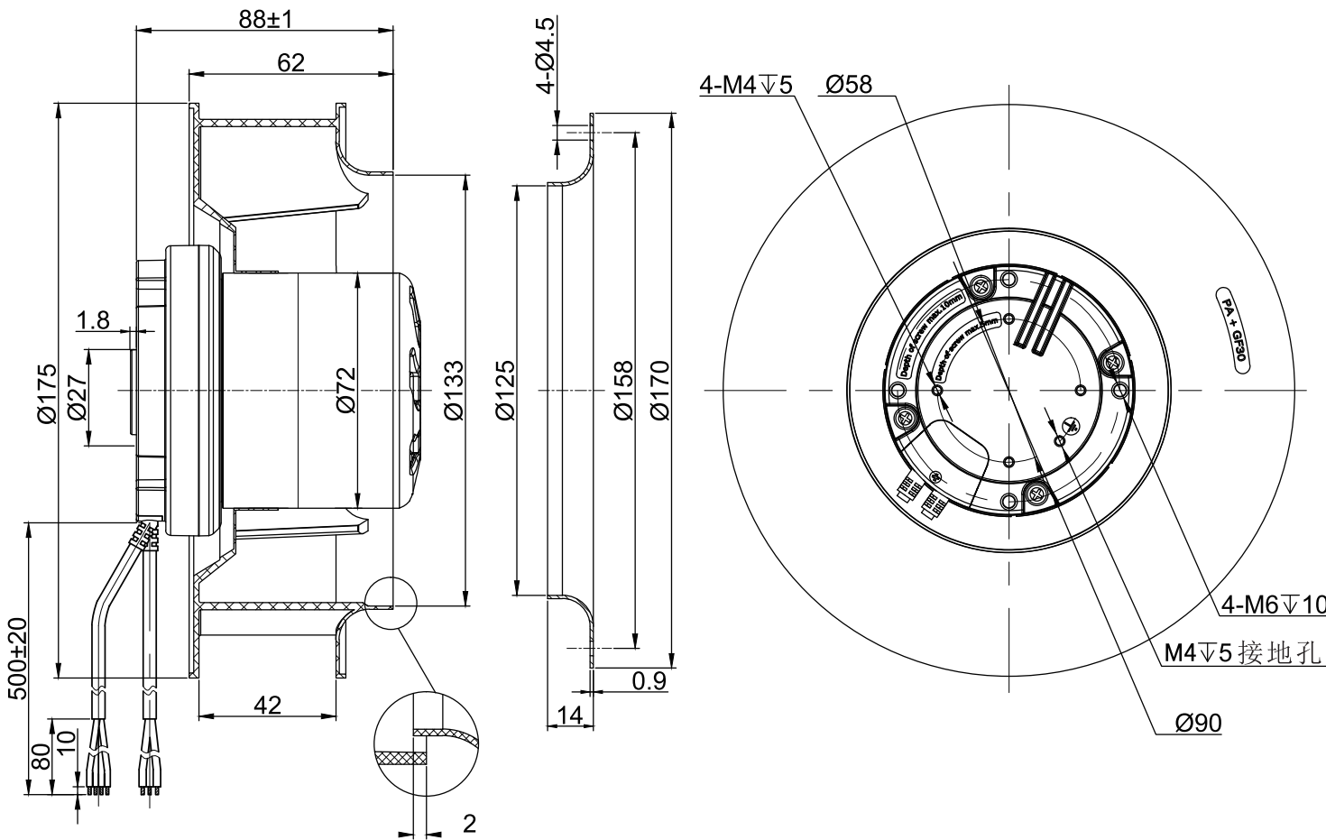
LWBE3G175-72PS-04 (with bracket)
