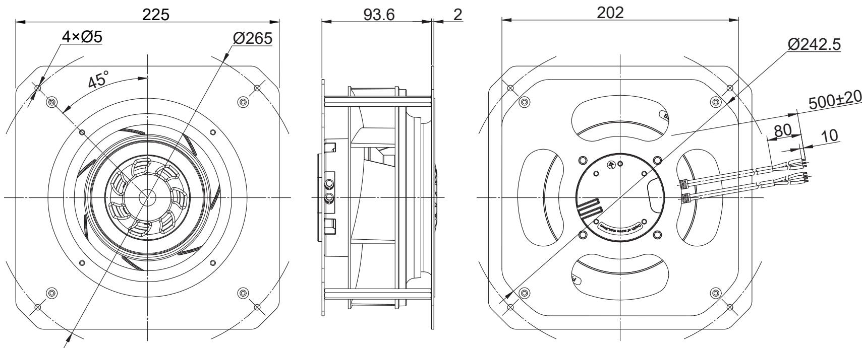
LWBE3G175-72PS-04 (with bracket)
