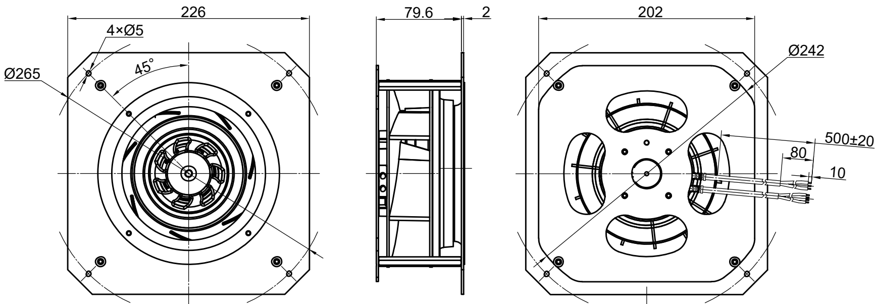
LWBE3G175-72PS-01 (with bracket)
