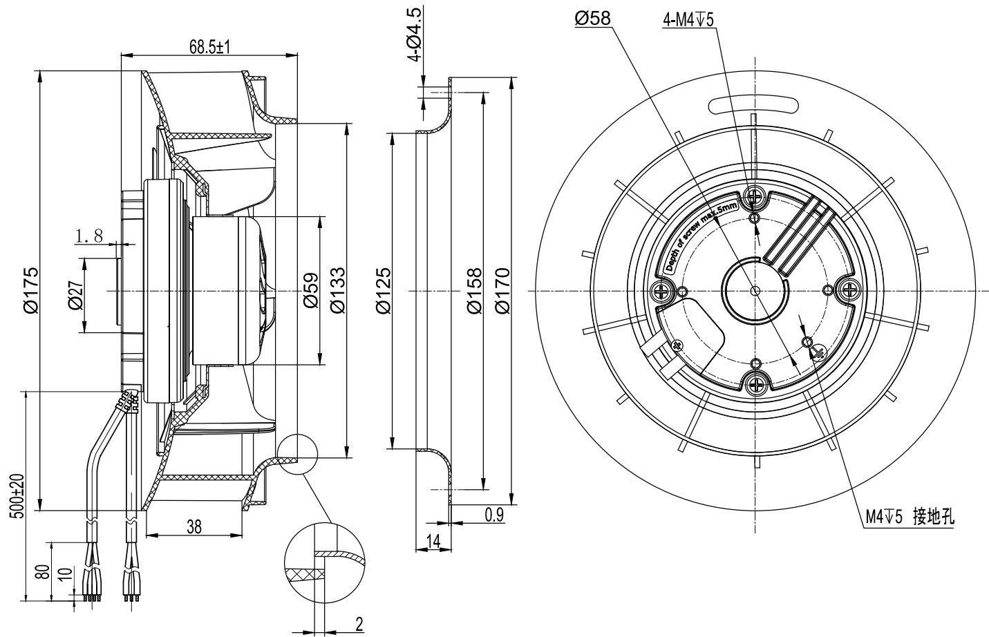
LWBE3G175-72PS-01 (with bracket)
