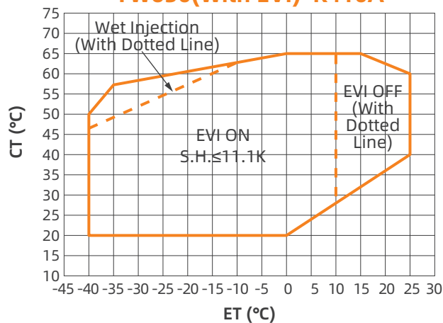
YW630(With EVI) R410A
