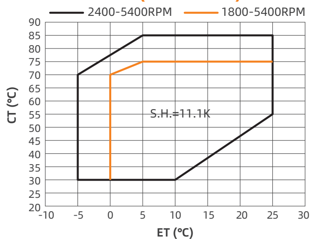
YIW60-72(Without EVI) R134a
