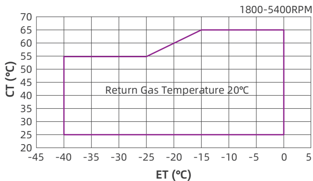
YIF38-72 R404A
