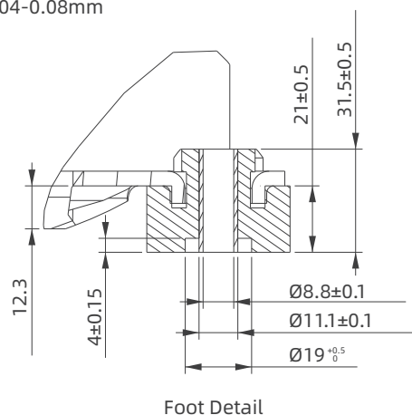
Foot Detail
