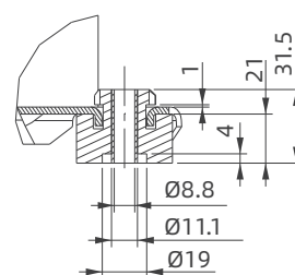
Mounting Feet
