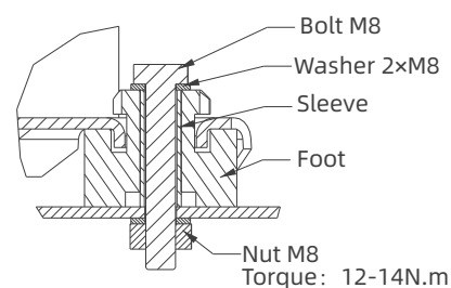
Foot installation recommendation
