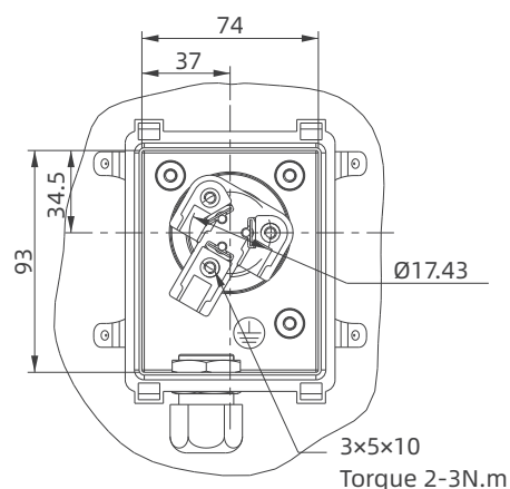
Wring diagram
