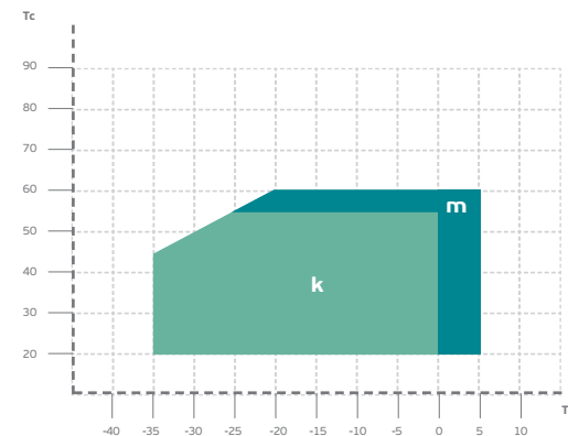
L/MBP R290/R134a/R600a
